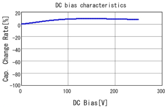
■ DE1E3KX152MB4BN01F C-DC bias capchange, 20.0degC, AC1
