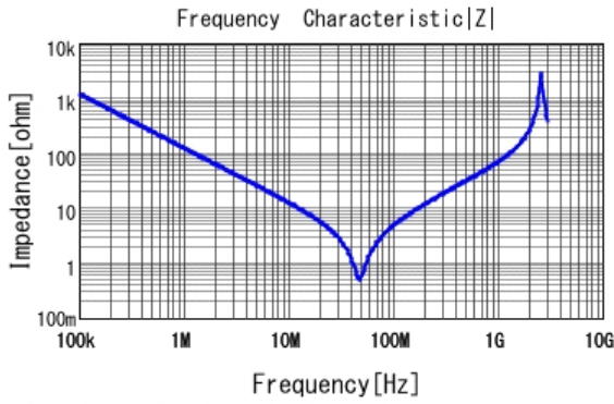
■ DE1E3KX152MB4BN01F |Z| DCOV, 20degC
