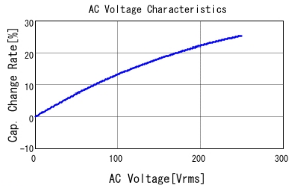
■ DE1E3KX152MB4BN01F C-AC Voltage capchange, DCOV, 20.0
