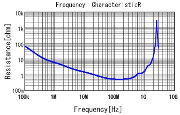
■ DE1E3KX102MN4AP01F R DCOV, 20degC
