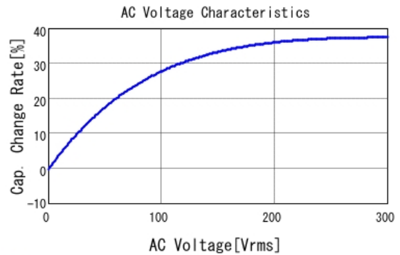
■ DE1E3KX102MN4AP01F C-AC Voltage capchange, DCOV, 20.0
