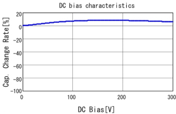
■ DE1E3KX102MN4AP01F C-DC bias capchange, 20.0degC, AC1
