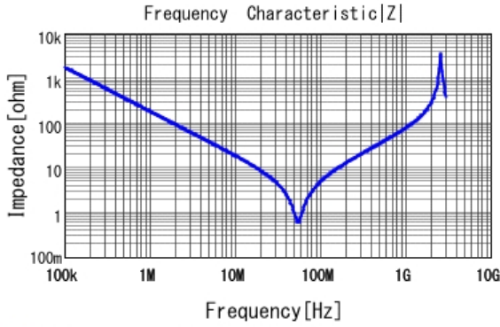
■ DE1E3KX102MN4AP01F |Z| DCOV, 20degC
