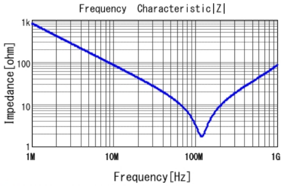
■ DE1B3RA221KN4AN01F |Z| DCOV, 20degC
