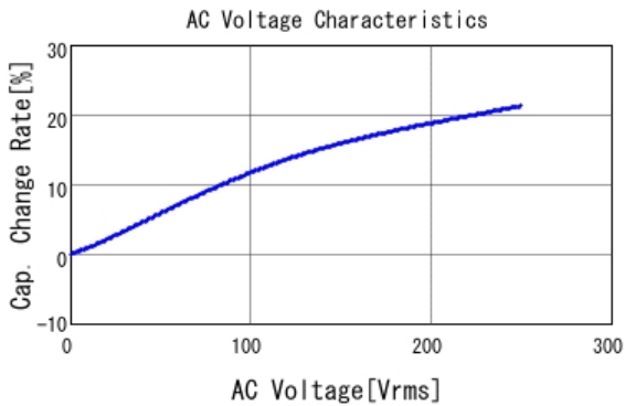
■ DE1B3RA221KN4AN01F C-AC Voltage capchange, DCOV, 20.0
