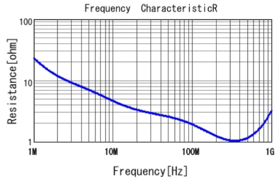
■ DE1B3RA221KN4AN01F R DCOV, 20degC
