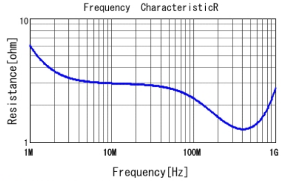
■ DE1B3RA101KA4BN01F R DCOV, 20degC
