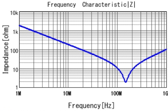
■ DE1B3RA101KA4BN01F |Z| DCOV, 20degC
