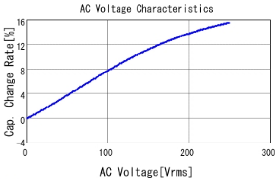
■ DE1B3RA101KA4BN01F C-AC Voltage capchange, DCOV, 20.0
