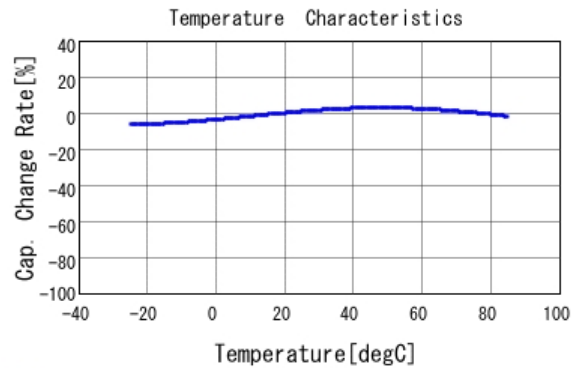
■ DE1B3RA101KA4BN01F C-Temp. capchange, DCOV, AC1Vrms
