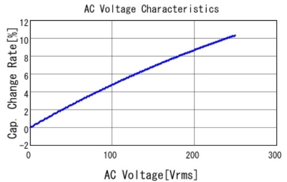
■ DE1B3KX101KN4AN01F C-AC Voltage capchange, DCOV, 20.0
