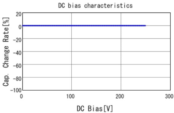
■ DE1B3KX101KN4AN01F C-DC bias capchange, 20.0degC, AC1
