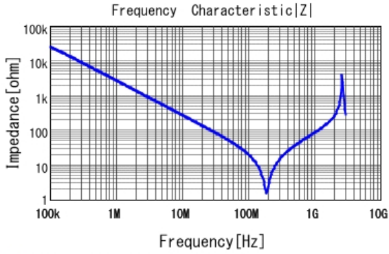
■ DE1B3KX101KN4AN01F |Z| DCOV, 20degC
