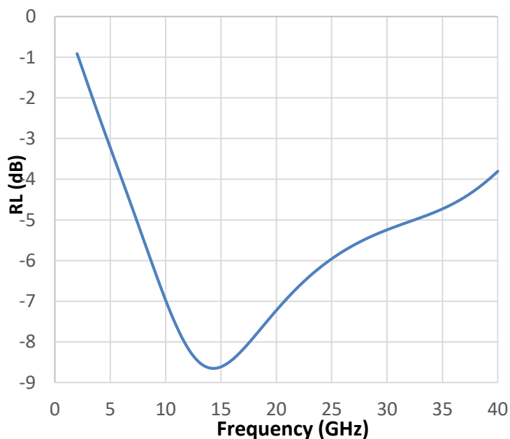
Reflection Loss
