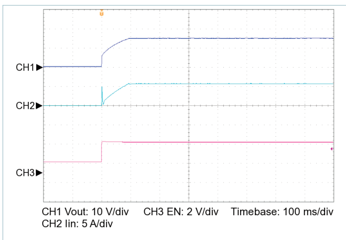
Figure 17 — Startup from EN, V_{IN} = 30\text{ V} , C_{OUT\_EXT} = 10000\ \mu\text{F} , R_{LOAD} = 1.402\ \Omega
