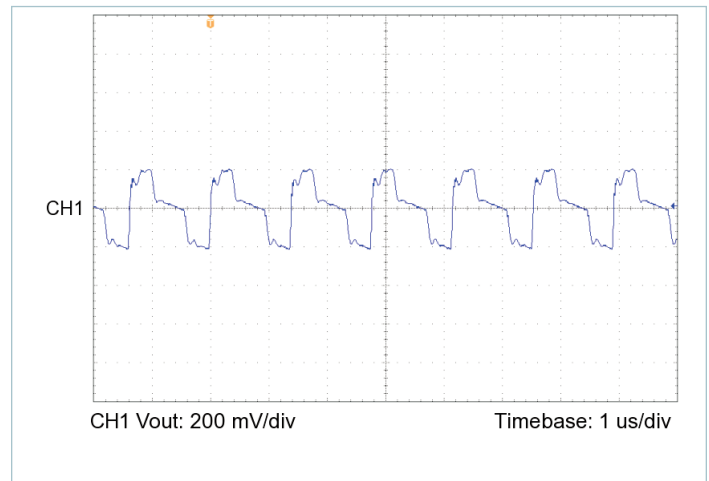
Figure 19 — Output voltage ripple, V_{IN} = 30\text{ V} , V_{OUT} = 15.0\text{ V} , C_{OUT\_EXT} = 1000\ \mu\text{F} , R_{LOAD} = 1.402\ \Omega
