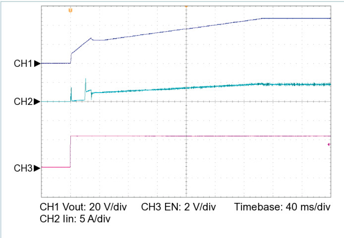
Figure 15 — Startup from EN, V_{IN} = 48\text{ V} , C_{OUT\_EXT} = 2200\ \mu\text{F} , R_{LOAD} = 7.200\ \Omega
