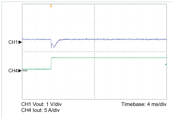
Figure 6 — 10% to 100% load transient response, V_{IN} = 48\text{ V} , nominal trim, C_{OUT\_EXT} = 220\ \mu\text{F}
