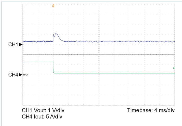
Figure 5 — 100% to 10% load transient response, V_{IN} = 48\text{ V} , nominal trim, C_{OUT\_EXT} = 220\ \mu\text{F}
