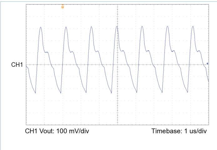
Figure 17 — Output voltage ripple, V_{IN} = 48\text{ V} , V_{OUT} = 48.0\text{ V} , C_{OUT\_EXT} = 220\ \mu\text{F} , R_{LOAD} = 7.200\ \Omega
