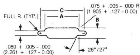
Figure 2: Rear Mounting
