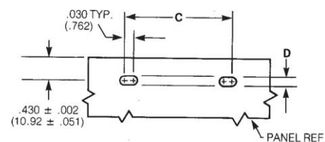
Figure 3: Edgeboard Mounting
