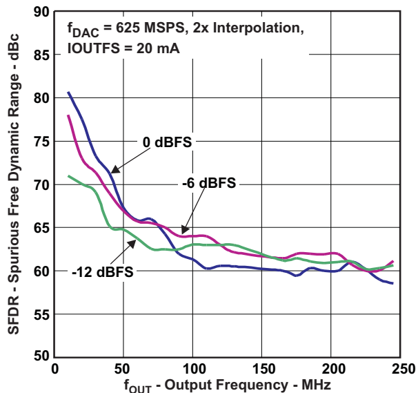
Figure 3. SFDR vs Input Scale
