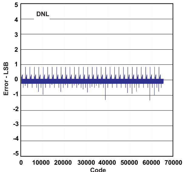
Figure 2. Differential Non-Linearity
