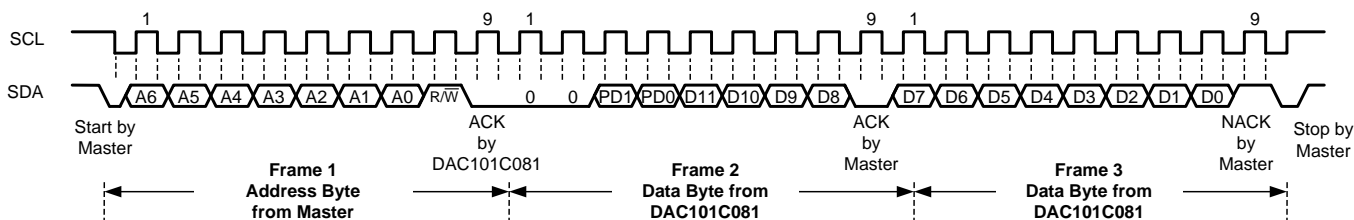
Figure 27. Typical Read from the DAC Register
