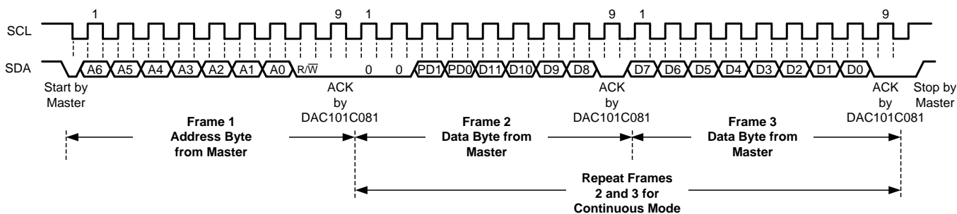
Figure 26. Typical Write to the DAC Register
