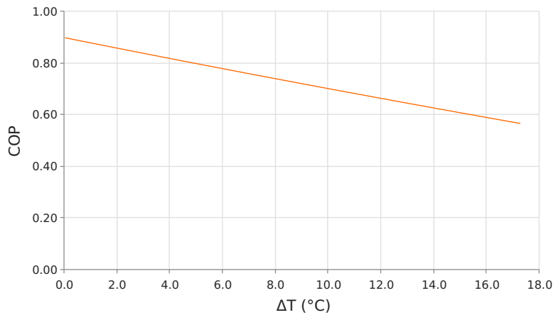
Coefficient of Performance (COP = Qc/Pin) Voperating = 24 Volts | Ioperating = 3.3 Amps
