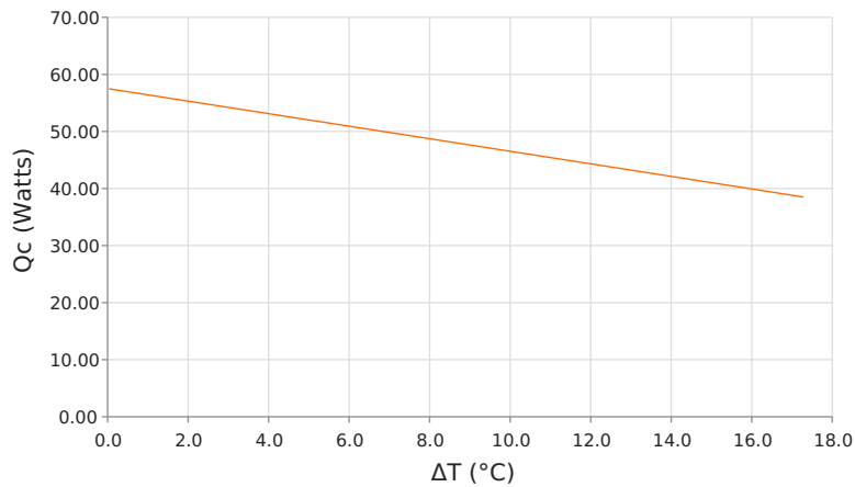
Heat Pumped at Cold Side (Qc) Voperating = 24 Volts | Ioperating = 3.3 Amps
