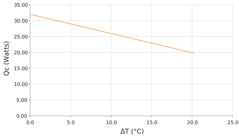
Heat Pumped at Cold Side (Qc) Voperating = 12 Volts | Ioperating = 3.5 Amps
