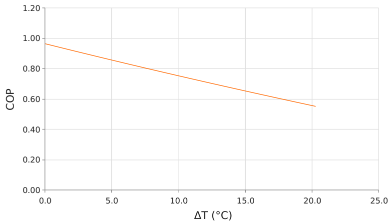
Coefficient of Performance (COP = Qc/Pin) Voperating = 12 Volts | Ioperating = 3.5 Amps
