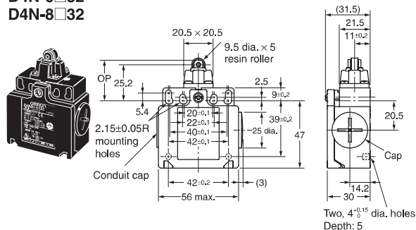
Roller Plunger D4N-6□32 D4N-8□32
