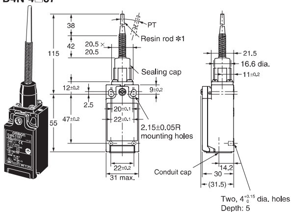
Plastic Rod *2 D4N-2□87 D4N-4□87
