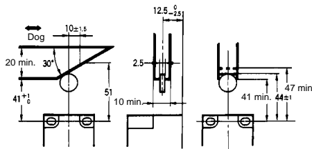
Roller Plunger (D4D-□□32N)
