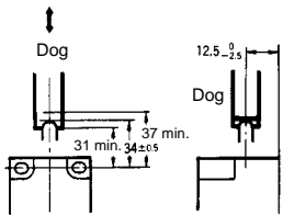
Sealed Plunger (D4D-□□31N)
