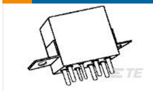
TE Part #3-1617758-0 FCB-205-0122M=M83536/1-022M
