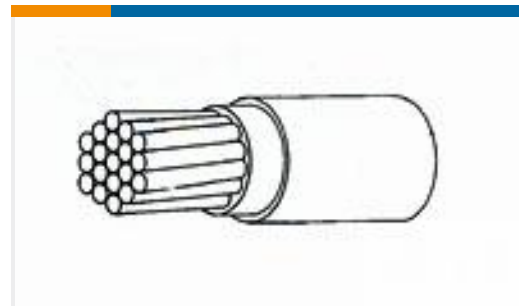
TE Part #218542-002 22759/34-24-9
