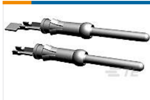
TE Part #1-66103-7 III+ PIN,24-20, 30AU/SN,SMPACK
