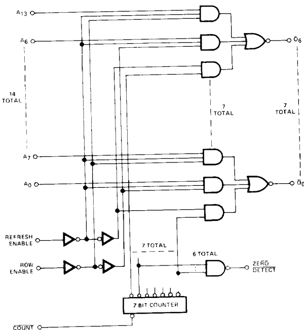
LOGIC DIAGRAM
