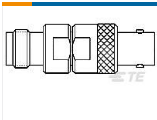
TE Part #1057845-1 3180 2320 00
