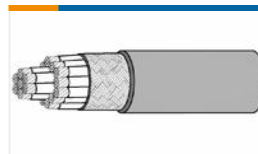
TE Part #7103033001 VG-95218-T025-G007
