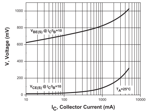
"ON" Voltage
