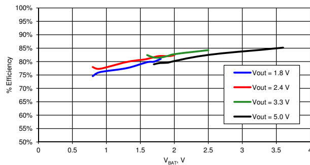
Figure 11-12. Efficiency vs V_{BAT} , L_{BOOST} = 10 \mu H [32]
