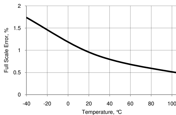
Figure 11-66. VDAC Full Scale Error vs Temperature, 4 V Mode
