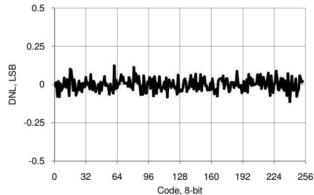
Figure 11-50. IDAC DNL vs Input Code, Range = 255 \mu A, Sink Mode
