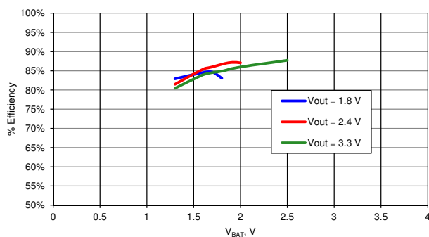
Figure 11-13. Efficiency vs V_{BAT} , L_{BOOST} = 22 \mu H [32]
