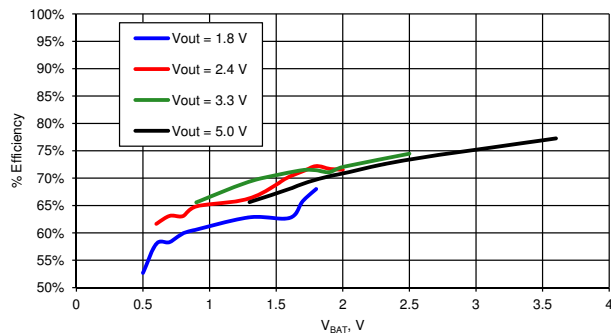
Figure 11-11. Efficiency vs V_{BAT} , L_{BOOST} = 4.7 \mu H [32]
