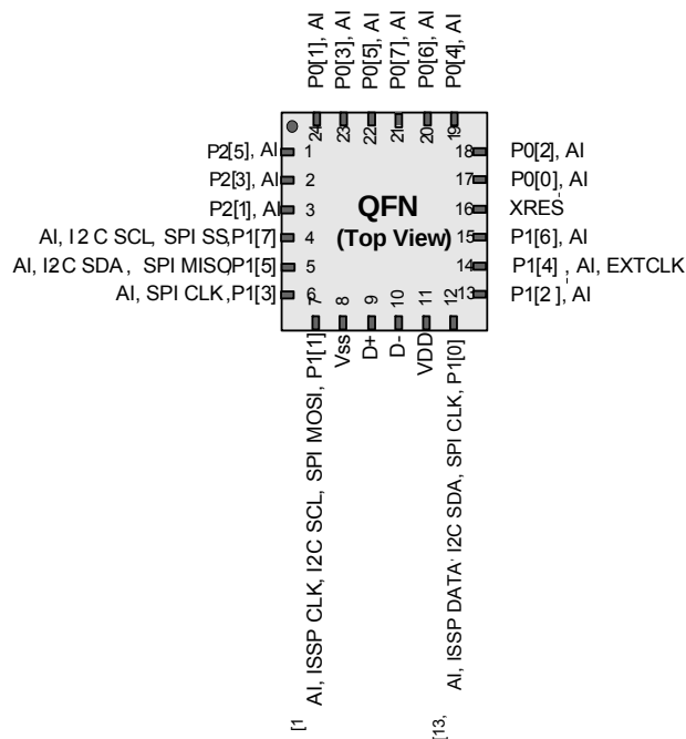
Figure 4. CY8C20396A
