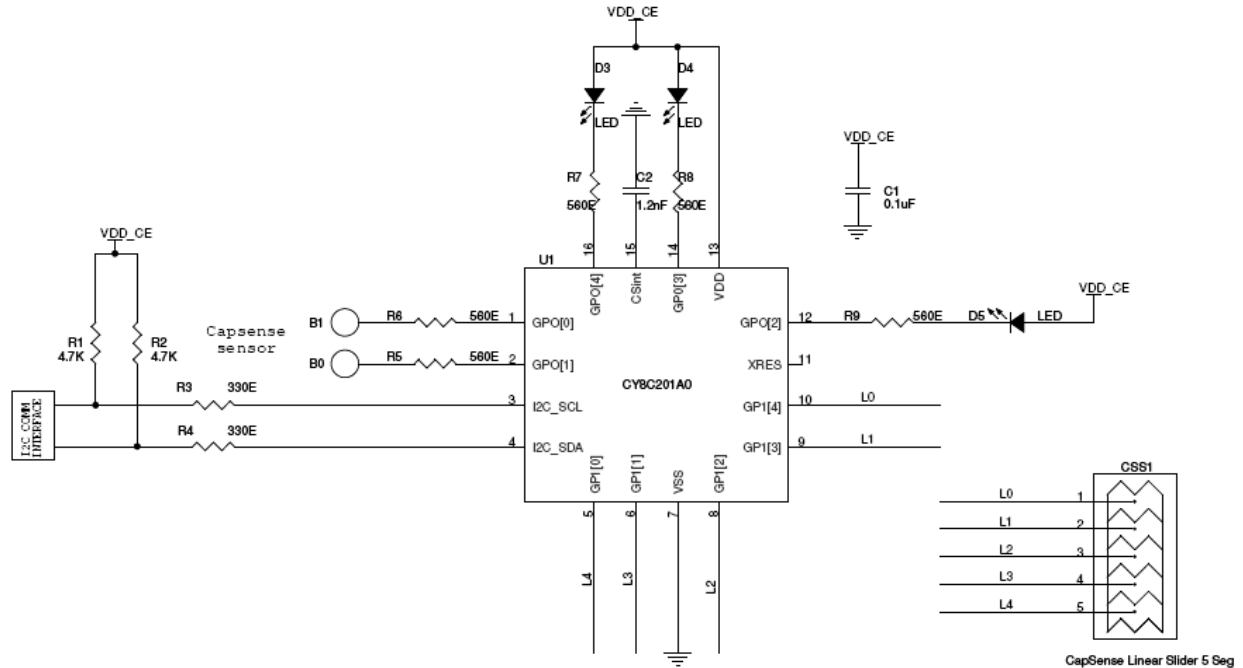
Figure 4. Circuit 2 – Compatibility with 1.8 V I 2 C Signaling [4, 5]
