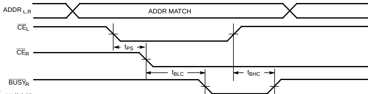
Figure 9. Busy Timing Diagram No. 1 ( \overline{\text{CE}} Arbitration) [38]
