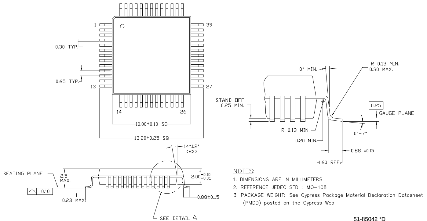
Figure 14. 52-pin PQFP (10 × 10 × 2.0 mm) N5210 Package Outline, 51-85042
