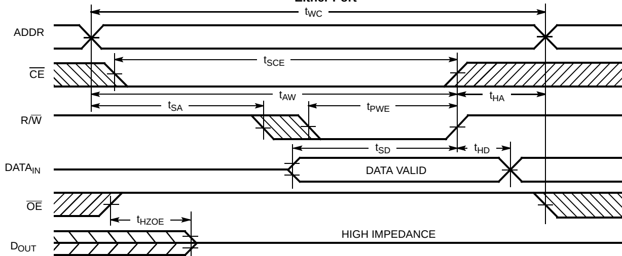
Figure 6. Write Cycle No. 1 ( \overline{\text{OE}} Three-States Data I/Os – Either Port) [31, 32]
