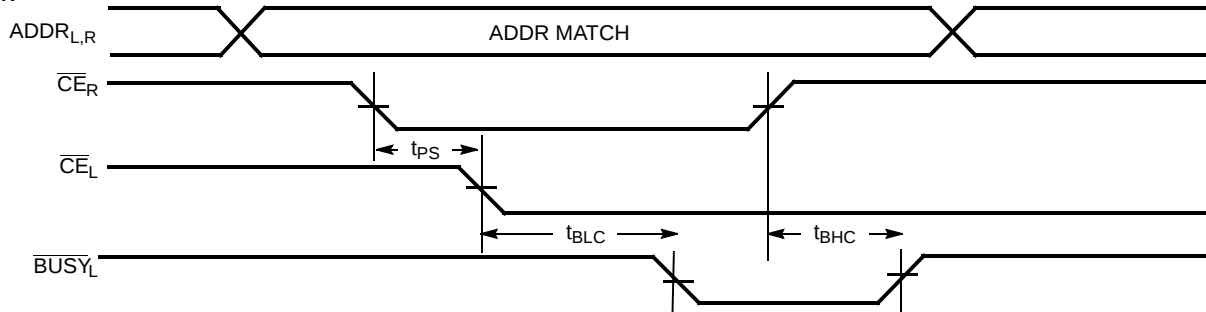
Figure 10. Busy Timing Diagram No. 2 (ADDR Arbitration) [38]
