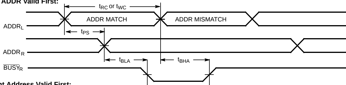
Figure 10. Busy Timing Diagram No. 2 (ADDR Arbitration) [38]
