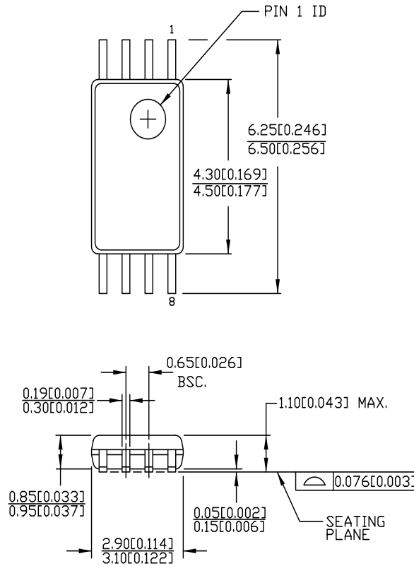
Figure 6. 8-pin TSSOP (4.40 mm Body) Z08.173/ZZ08.173, 51-85093
