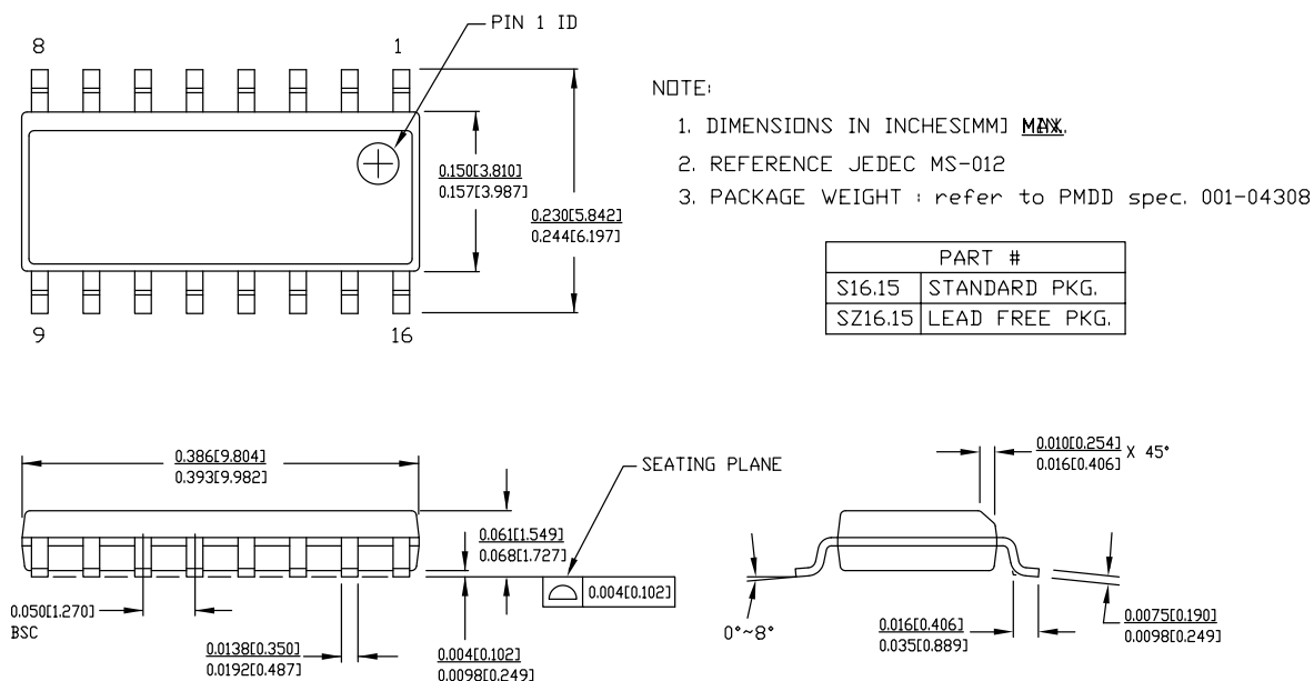
Figure 11. 16-pin SOIC (150 Mil) S16.15/SZ16.15 Package Outline, 51-85068
