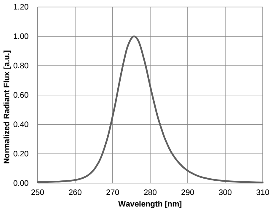
Fig 1. Spectrum, T_s=25^{\circ}\text{C} , I_F=600\text{mA}
