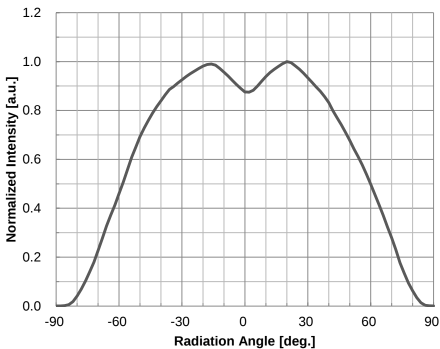
Fig 8. Typical Spatial Distribution, I_F=600\text{mA}
