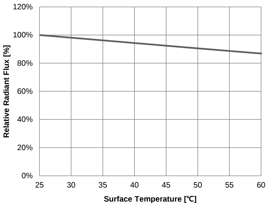
Fig 5. Surface Temperature vs. Relative Radiant Flux, I_F=600\text{mA}
