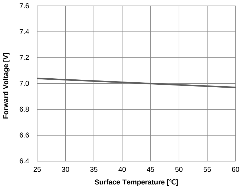
Fig 7. Surface Temperature vs. Forward Voltage, I_F=600\text{mA}
