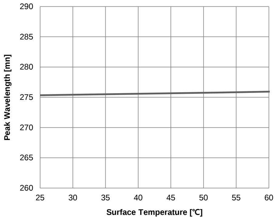
Fig 6. Surface Temperature vs. Peak Wavelength, I_F=600\text{mA}
