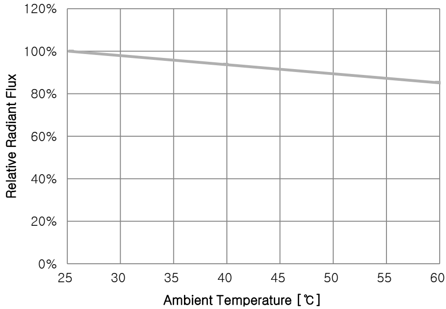
Fig 5. Ambient Temperature vs. Relative Radiant Flux, I_F=20mA
