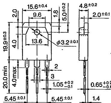
Outline Drawing Ⓢ67
