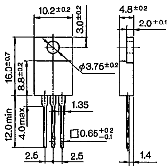
Outline Drawing Ⓢ66
