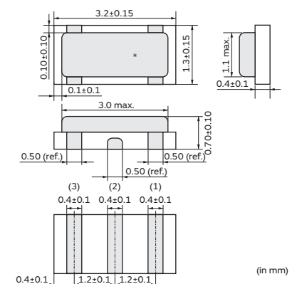
CSTCE_G_A 8.00-13.99MHz
