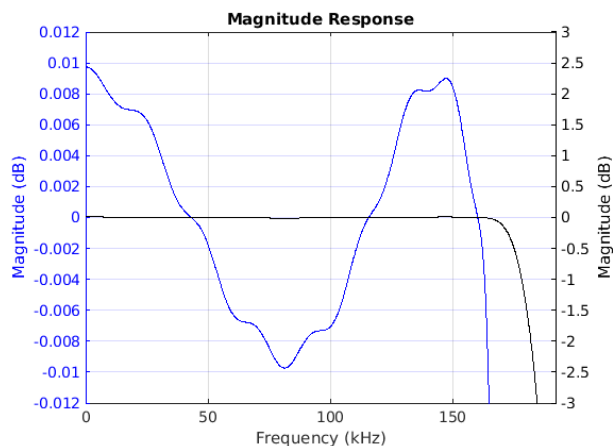
Figure 7-43. Passband Magnitude
