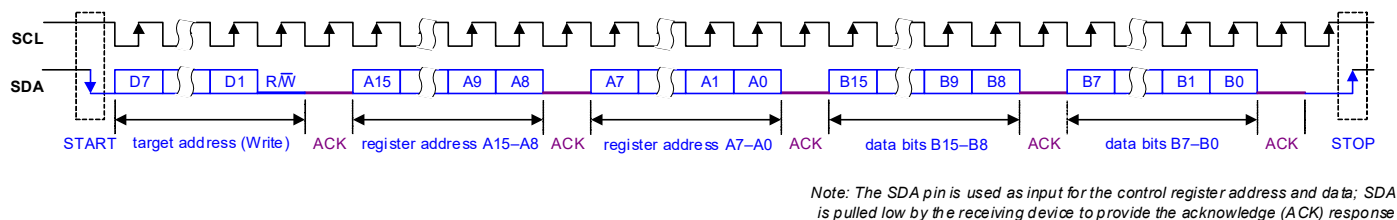
Figure 4-27. Control Interface I 2 C Register Write
