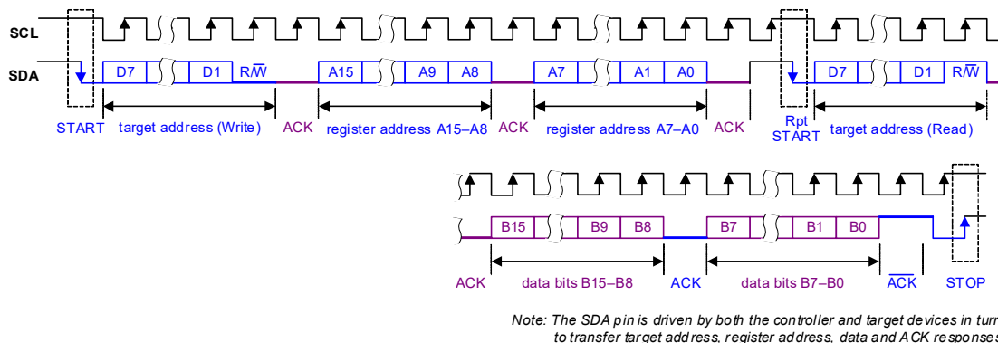
Figure 4-28. Control Interface I 2 C Register Read
