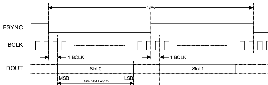
Figure 4-8. I 2 S Data Format
