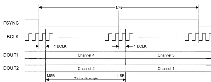
Figure 4-26. Reverse Channel Order
