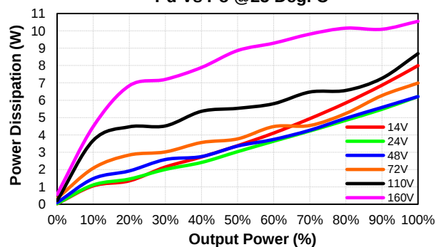
CQB50W12-72S48 Pd Vs Po @25 Deg. C
