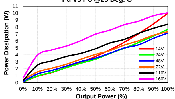
CQB50W12-72S12 Pd Vs Po @25 Deg. C
