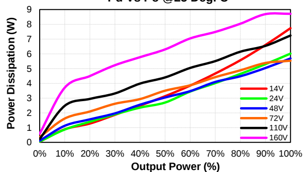
CQB50W12-72S24 Pd Vs Po @25 Deg. C
