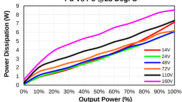
CQB50W12-72S05 Pd Vs Po @25 Deg. C
