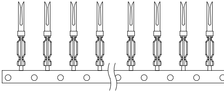
CPF STANDARD FEMALE CONTACTS, 24-28 AWG
