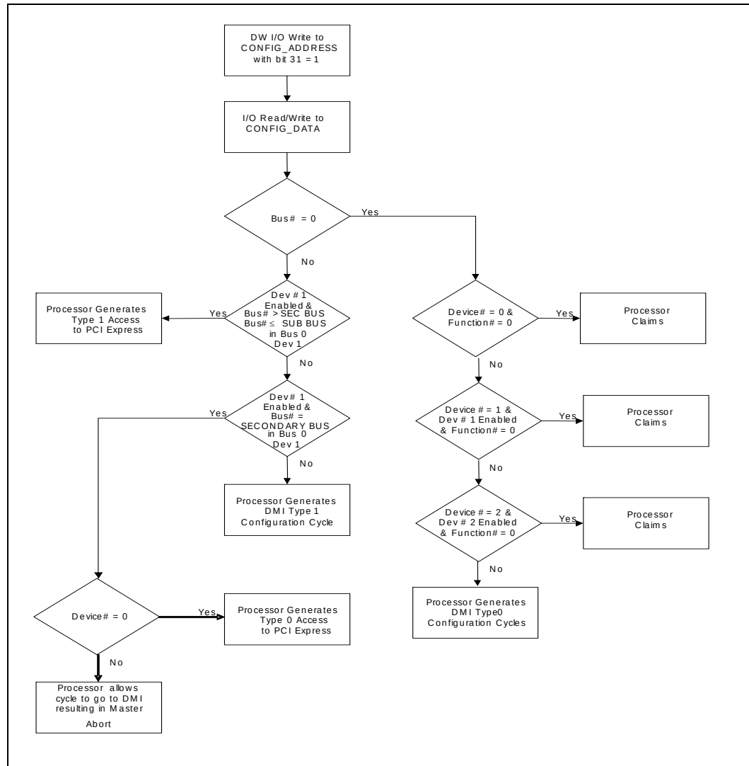
Figure 10. Processor Configuration Cycle Flow Chart
