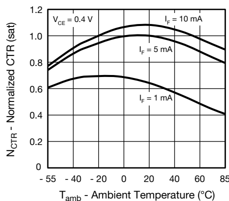
Fig. 11 - Normalized CTR (sat) vs. Ambient Temperature
