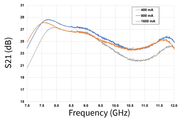
Figure 39. Gain vs Frequency as a Function of IDQ
