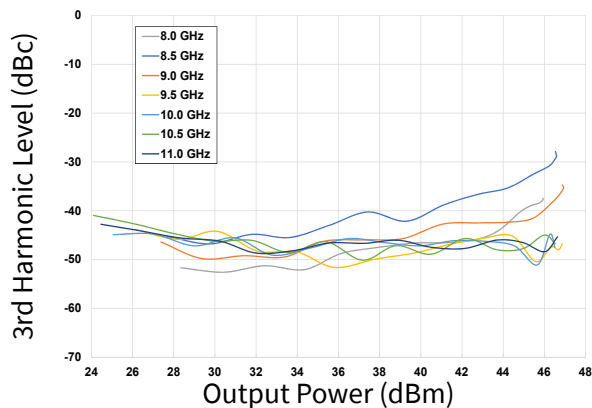
Figure 29. 3rd Harmonic vs Output Power as a Function of Frequency
