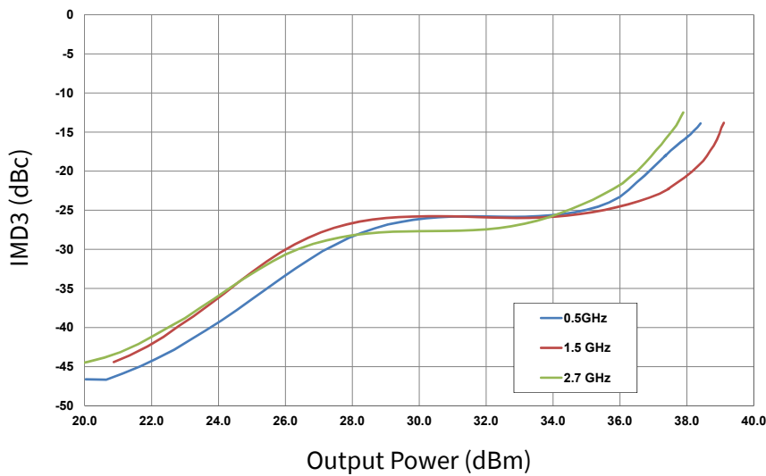
Figure 4. Third Order Intermodulation Distortion vs Output Power measured in demonstration amplifier circuit CMPA0527005F-AMP1 V_{DD} = 50\text{ V} , I_{DQ} = 0.110\text{ A} , T_{case} = 25^\circ\text{C} , \Delta f = 1\text{ MHz}
