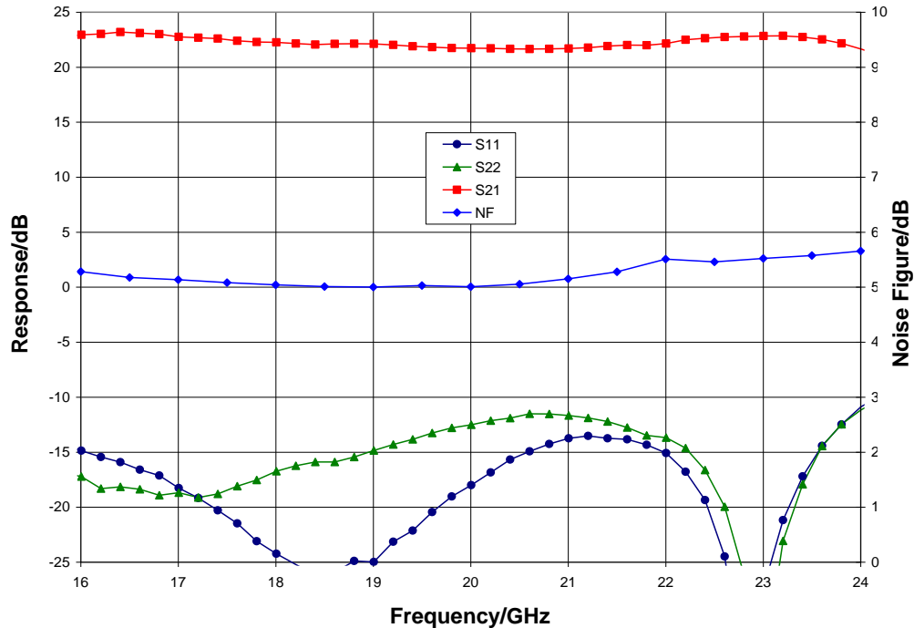
Narrow-band Performance, V_{dd} = 5\text{ V} , I_{dd} = 250\text{ mA} , T_A = 25^\circ\text{C}
