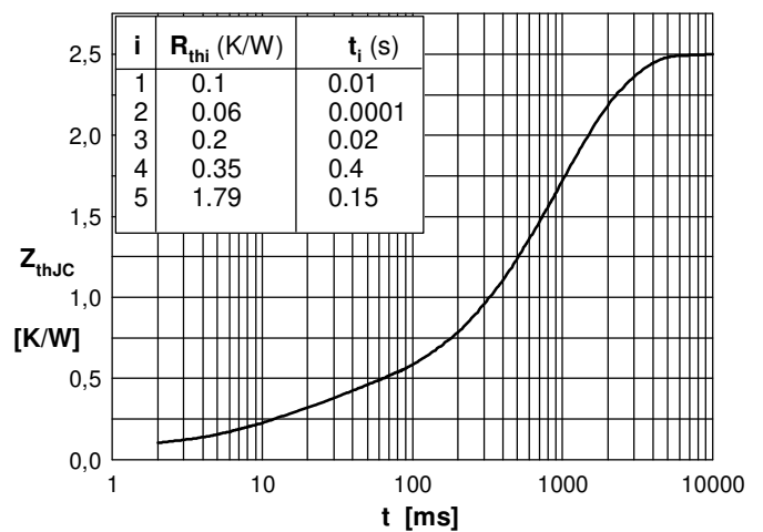
Fig. 7b Transient thermal impedance junction to case
