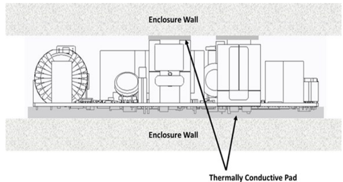
Fig. 3. Example of the CLP0612DC for sealed enclosure applications
