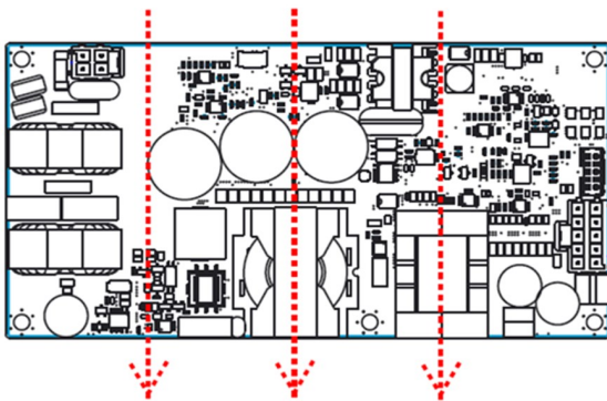
Fig. 2. Preferred airflow direction for cooling
