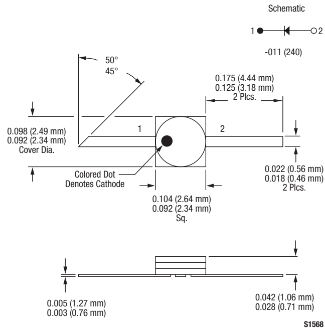
Figure 18. -240 Package
