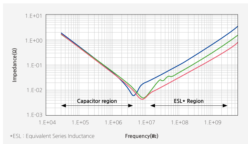
[Comparison between Impedance-Frequency Characteristics]
