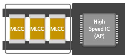
Multiple MLCC Used
