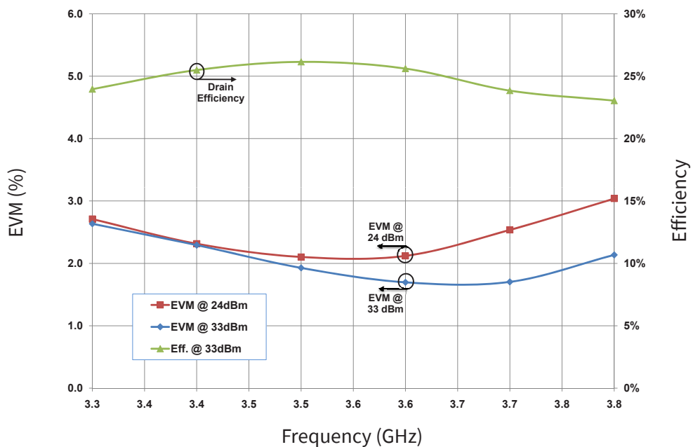
Figure 2. Typical EVM and Efficiency versus Frequency measured in the CGH35015F-AMP V_{DD} = 28\text{ V}, I_{DQ} = 100\text{ mA}, 802.16\text{-}2004\text{ OFDM}, \text{PAR} = 9.8\text{ dB}
