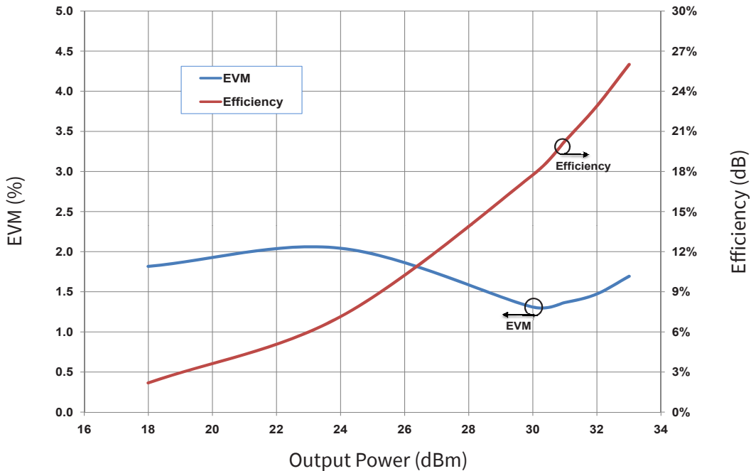
Figure 4. Typical EVM and Efficiency versus Power Output measured in the CGH35015F-AMP V_{DD} = 28\text{ V} , I_{DQ} = 100\text{ mA} , 802.16-2004 OFDM, PAR = 9.8 dB
