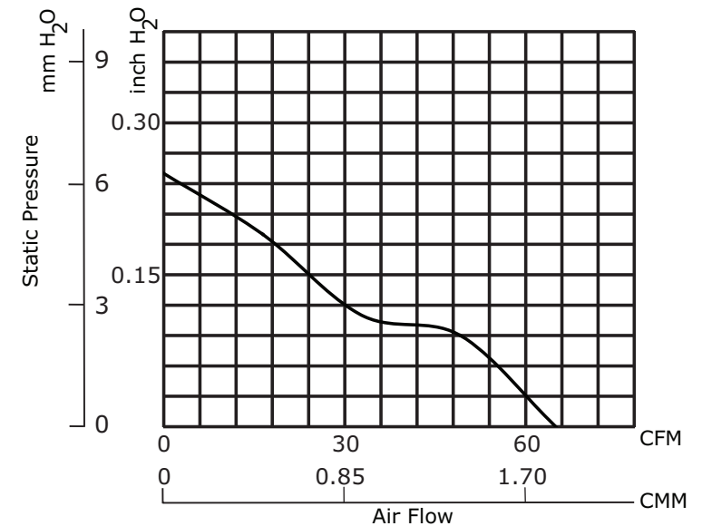
CFM-9225V-339-420
