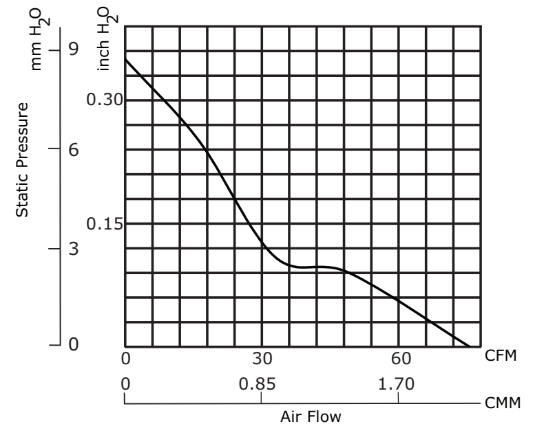
CFM-9225V-345-460
