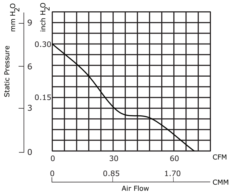
CFM-9225V-342-440
