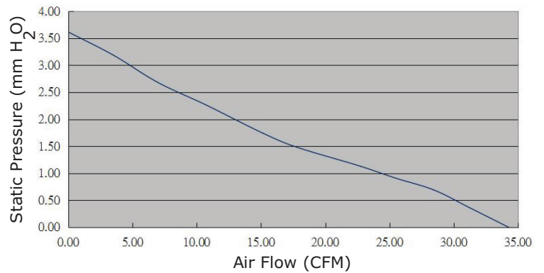
CFM-8020BF-235-346
