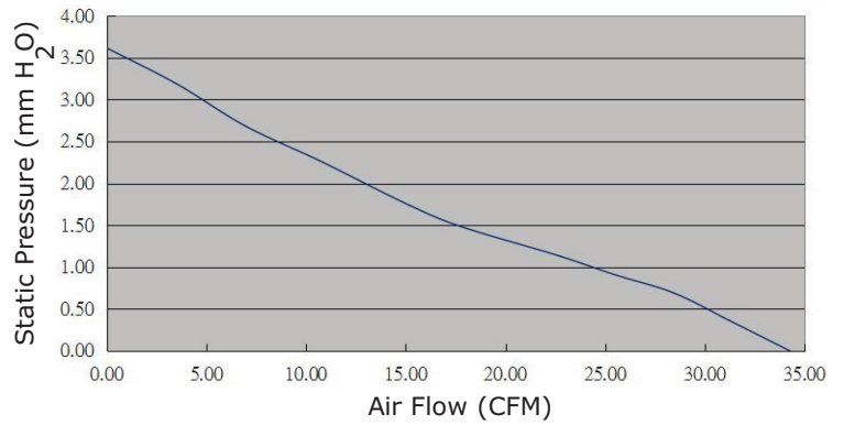
CFM-8020BF-155-444
