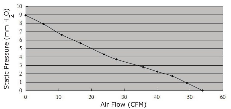
CFM-8020BF-235-346
