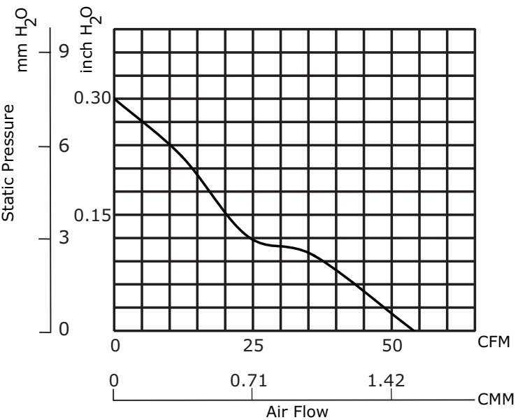
CFM-8025V-442-435
