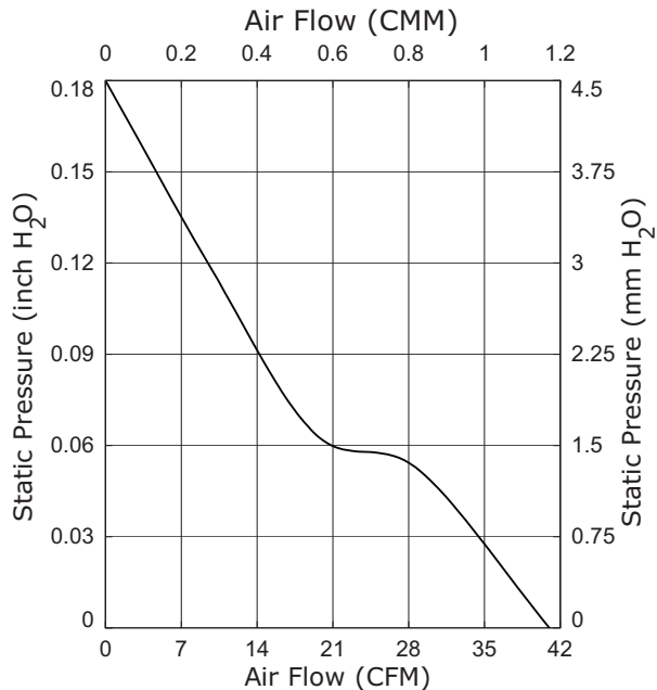
CFM-8025V-132-330
