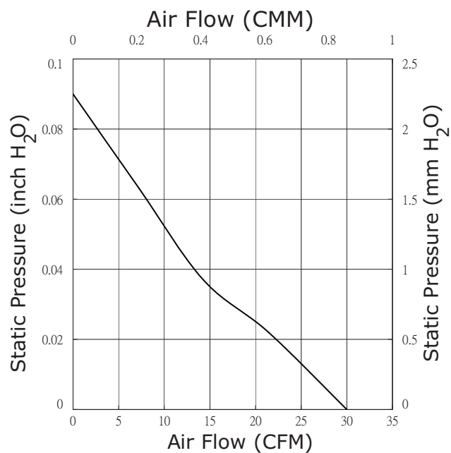
CFM-8015V-130-347
