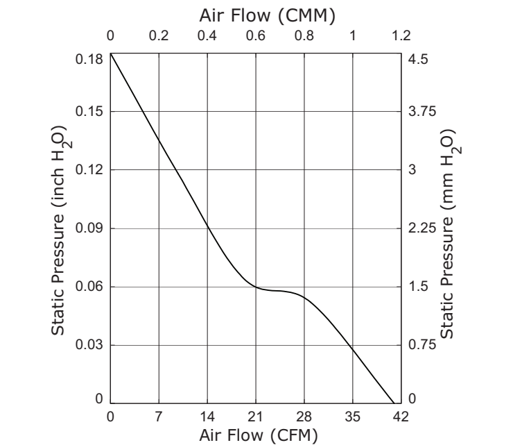
CFM-8025V-232-330
