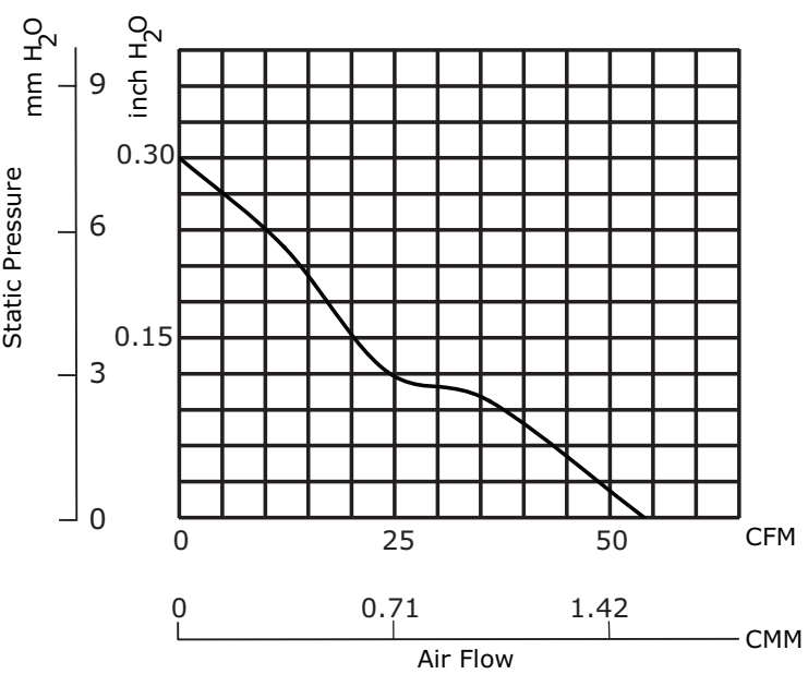
CFM-8025V-242-435
