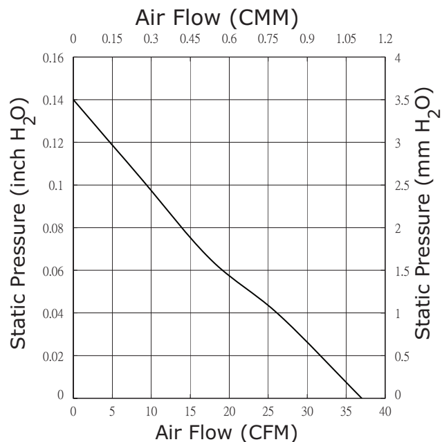
CFM-8015V-130-347
