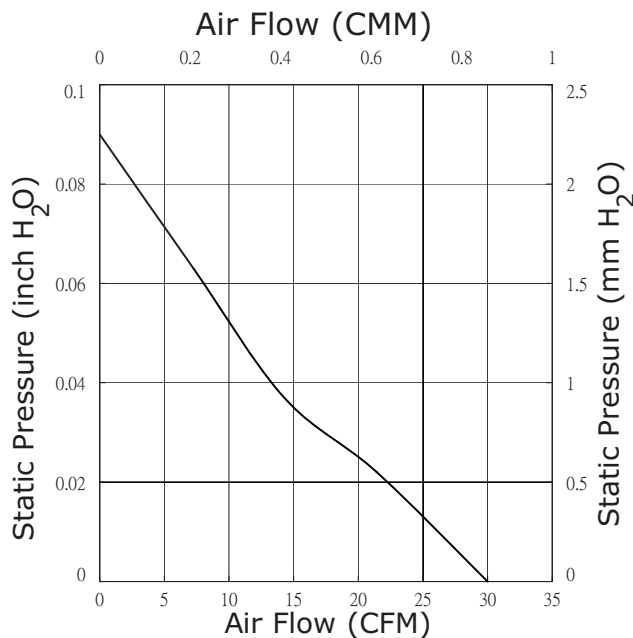
CFM-8015V-224-308
