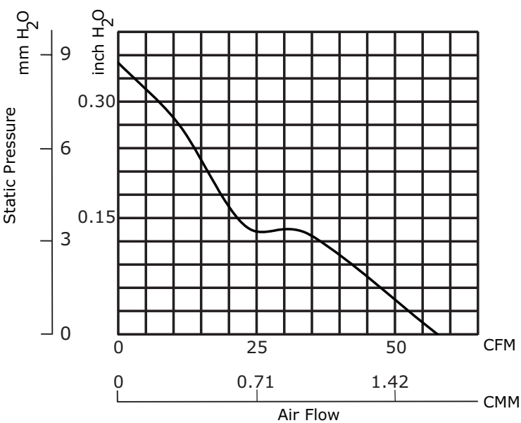
CFM-8025V-245-450
