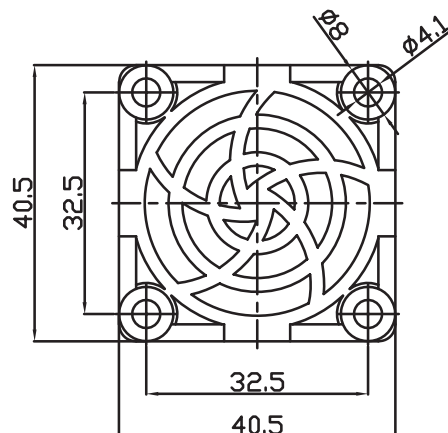
LOWER HOUSING
