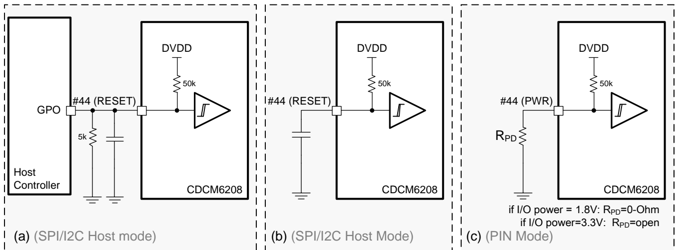
Figure 27. RESETN/PWR Pin Configurations
