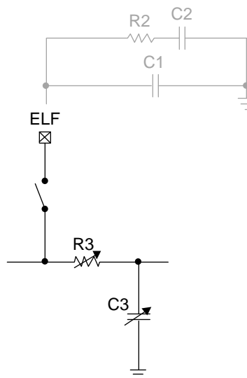
Figure 35. CDCM6208 PLL Loop Filter Topology
