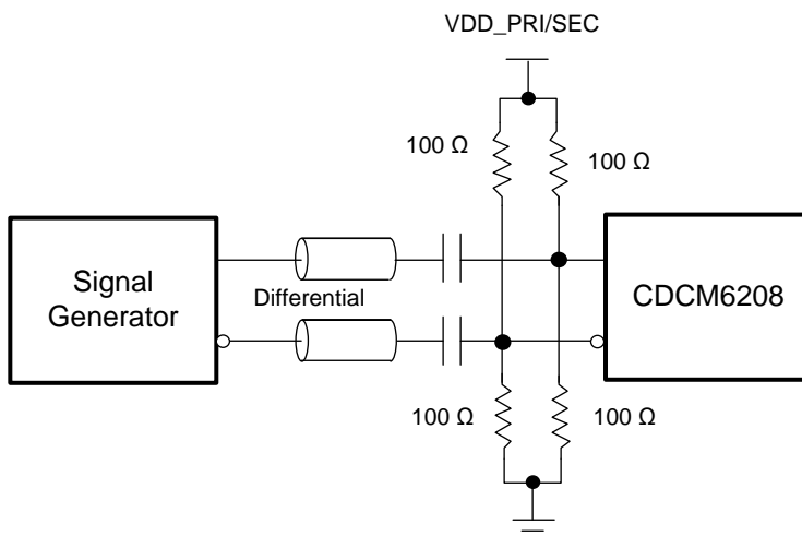
Figure 20. Differential Input AC Configuration During Device Test
