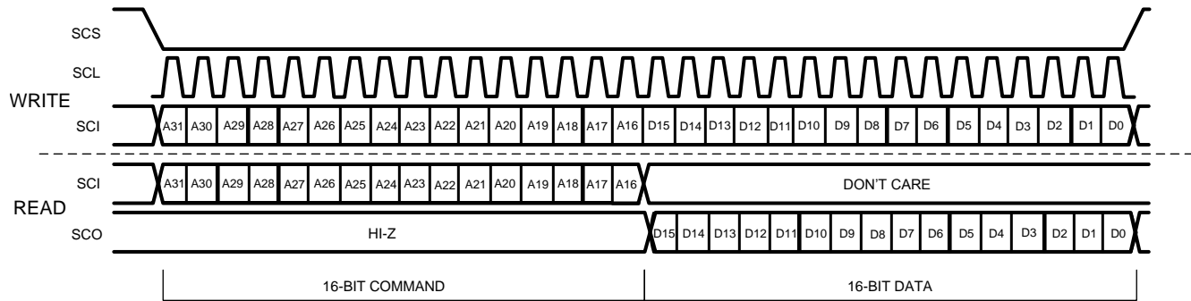
Figure 48. CDCM6208 SPI Port Message Sequencing
