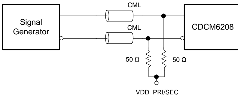
Figure 17. CML Input DC Configuration During Device Test
