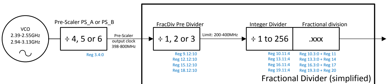
Figure 36. Fractional Output Divider Principle Architecture (Simplified Graphic, not Showing Output Divider Bypass Options)
