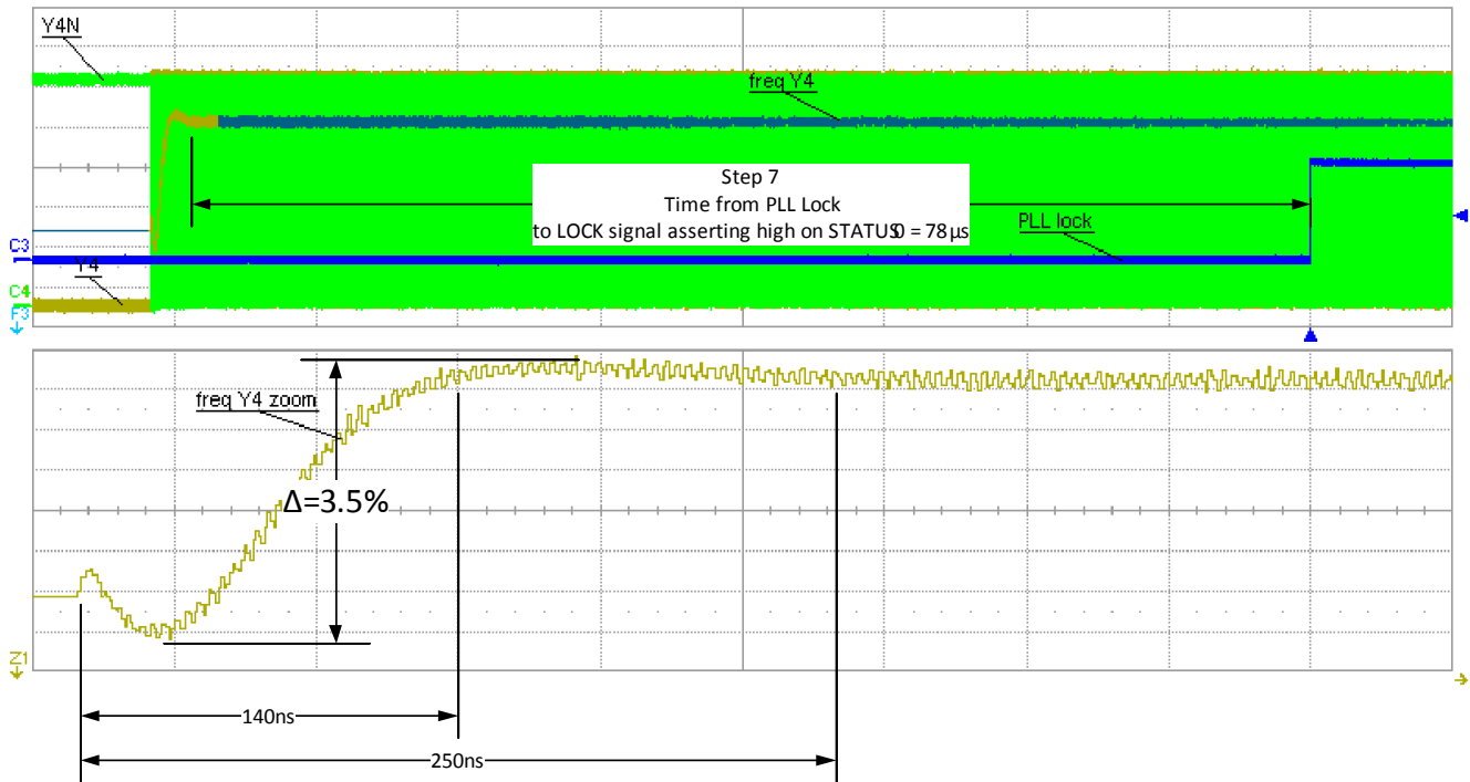
Figure 32. PLL Lock Behavior (Step 6)
