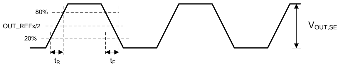
Figure 25. Single Ended Output Voltage and Rise and Fall Time
