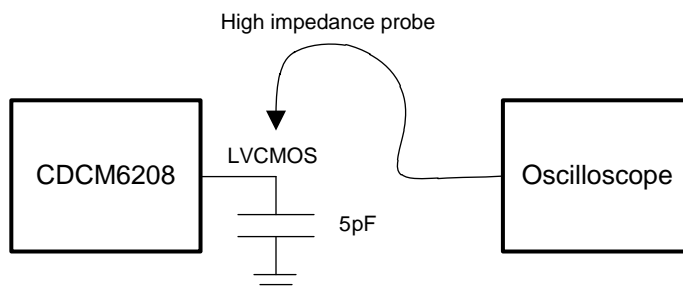
Figure 10. LVC MOS Output AC Configuration During Device Test ( V_{OH} , V_{OL} , t_{SLEW} )
