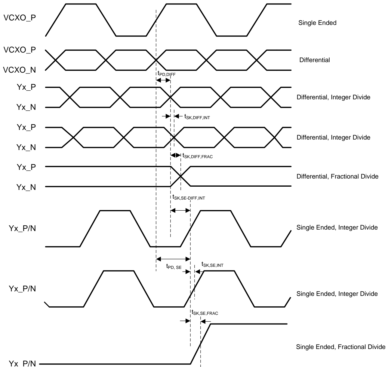
Figure 26. Differential and Single Ended Output Skew and Propagation Delay
