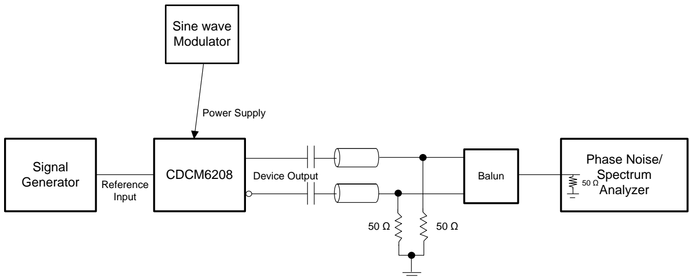
Figure 23. PSNR Test Setup
