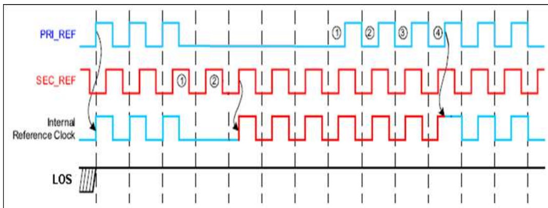
Figure 34. Smart Input MUX Auto-Switch Mode Timing Diagram
