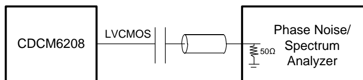
Figure 12. LVC MOS Output AC Configuration During Device Phase Noise Test
