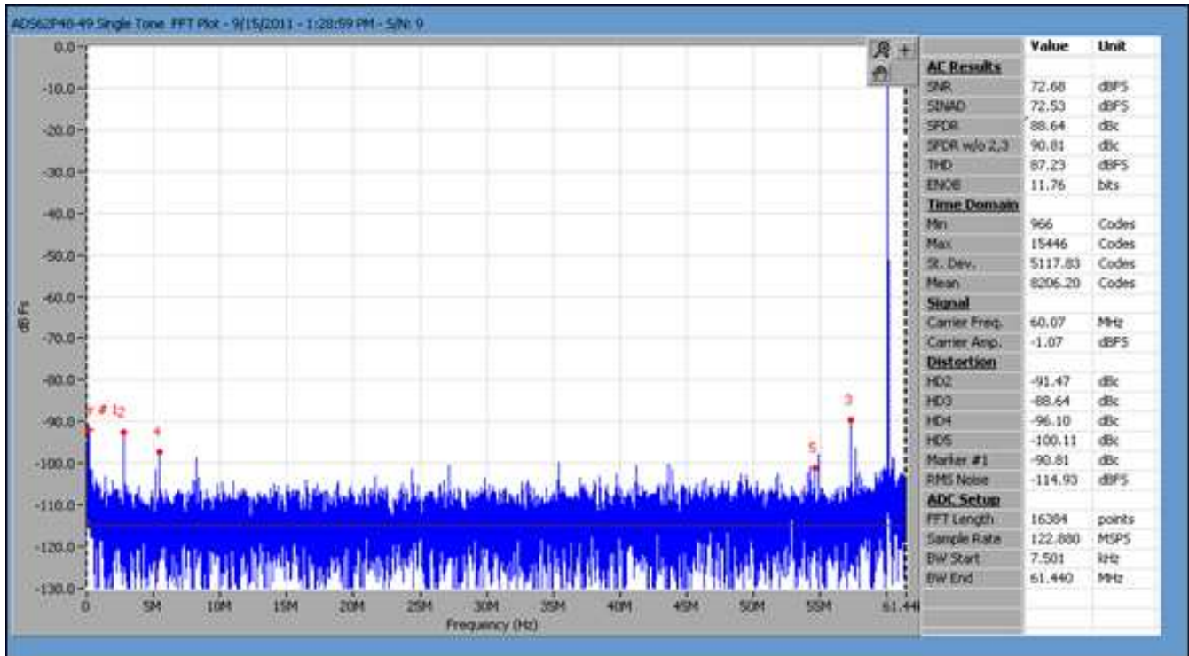
Figure 41. IF = 60 MHz Fclk = 122.88 MHz Baseline (Lab Clk Generator) ADC: ADS62P48-49
