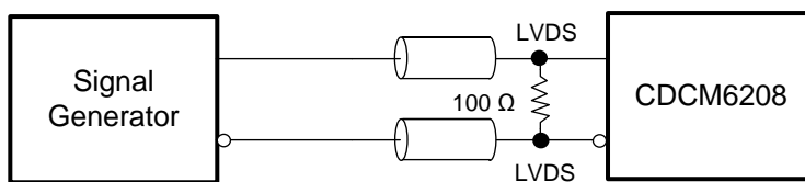
Figure 18. LVDS Input DC Configuration During Device Test
