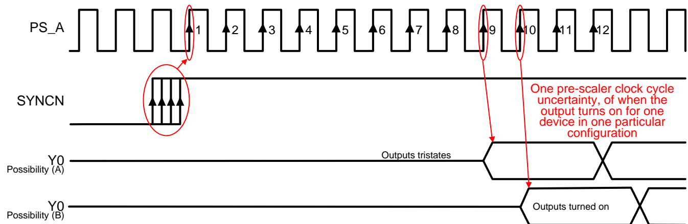
Figure 37. SYNCN to Output Delay Uncertainty
