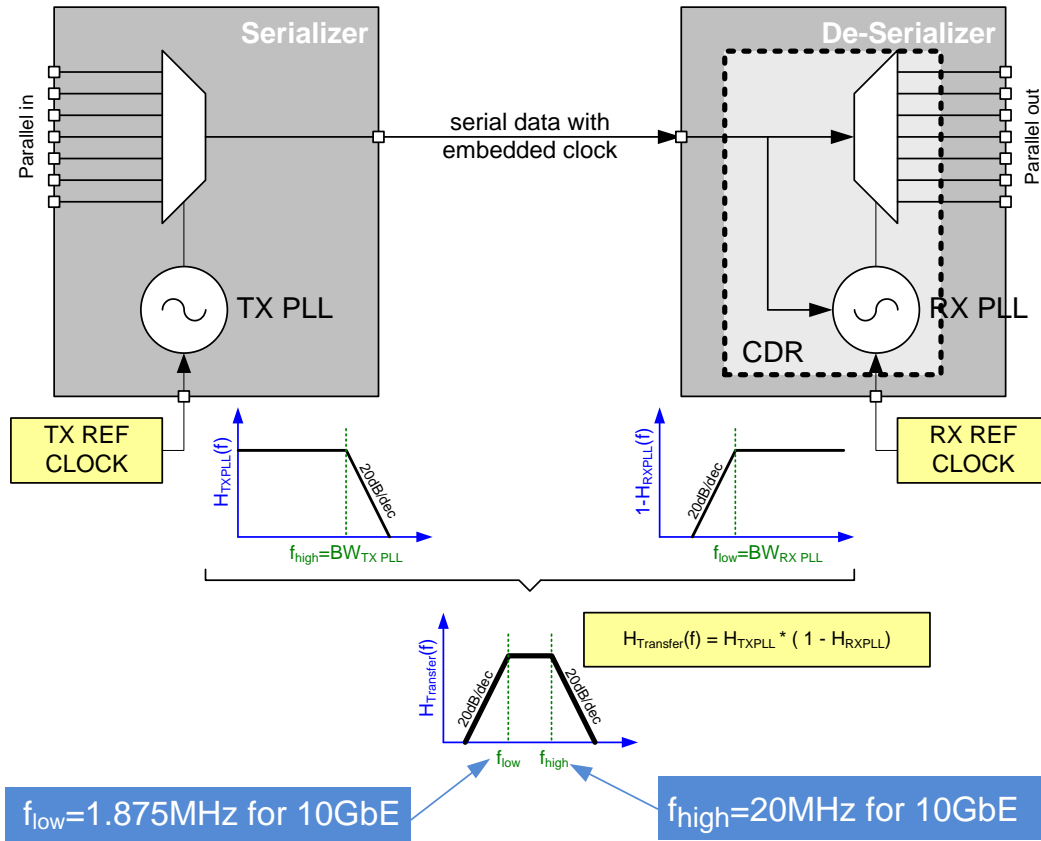
Figure 39. Serial Link Jitter Budget Explanation
