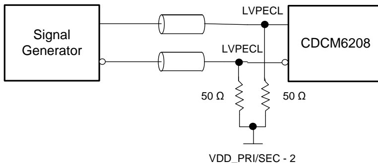
Figure 19. LVPECL Input DC Configuration During Device Test
