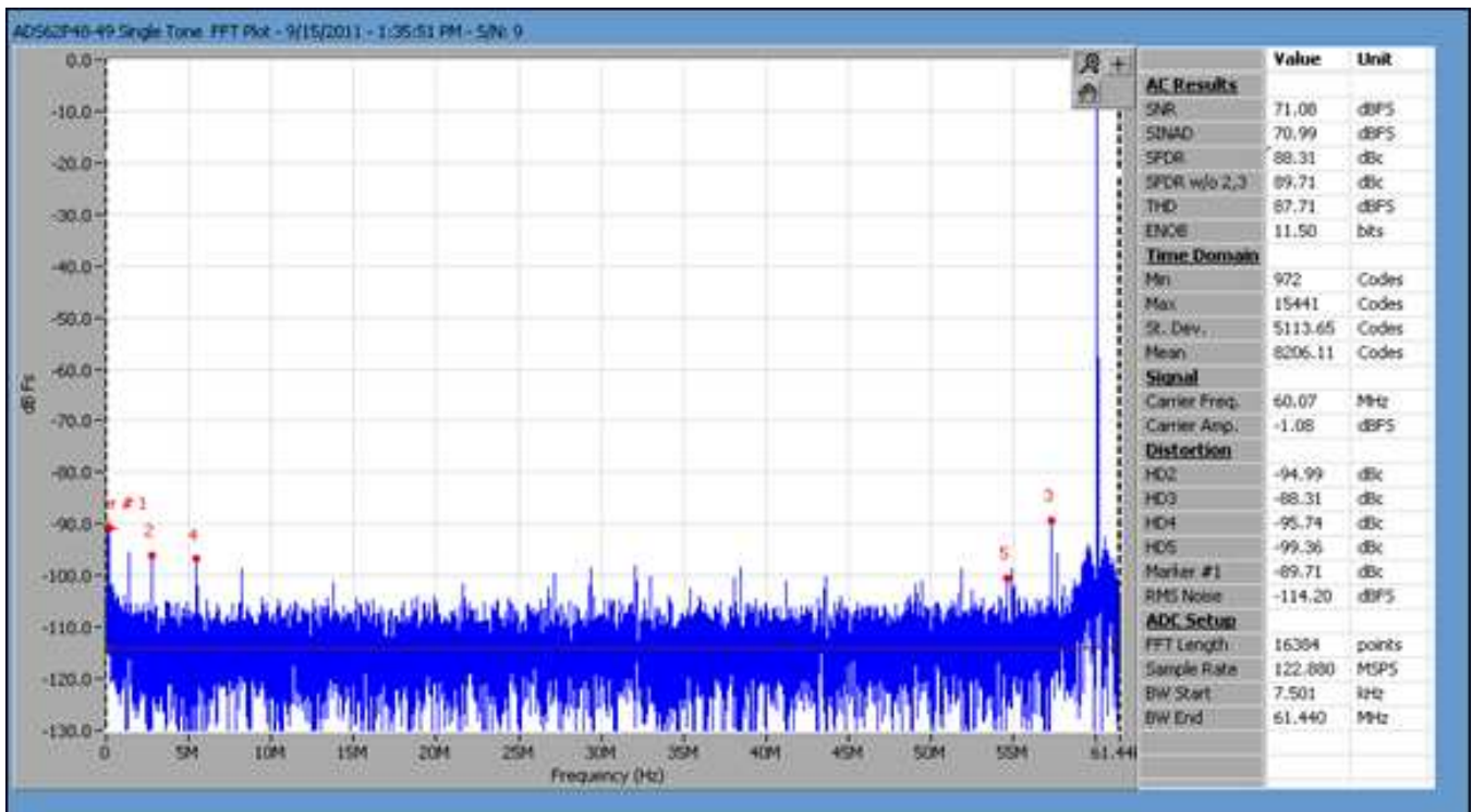
Figure 42. IF = 60 MHz Fclk = 122.88 MHz CDCM6208 driving ADC
