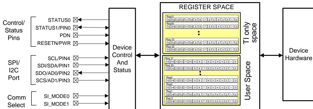
Figure 44. CDCM6208 Interface and Control Block
