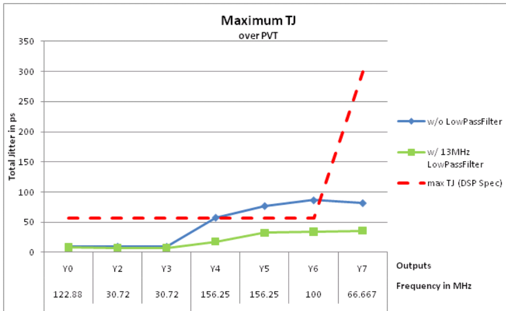
Figure 40. Maximum Jitter Over PVT
