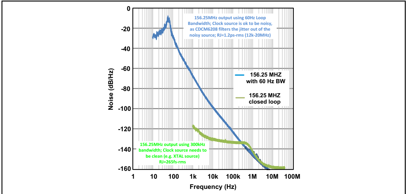
Figure 3. Phase Noise Plot for Jitter Cleaning Mode (blue) and Synthesizer Mode (green)
