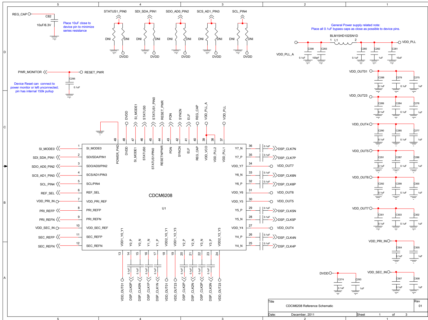
Figure 54. Schematic Page 1
