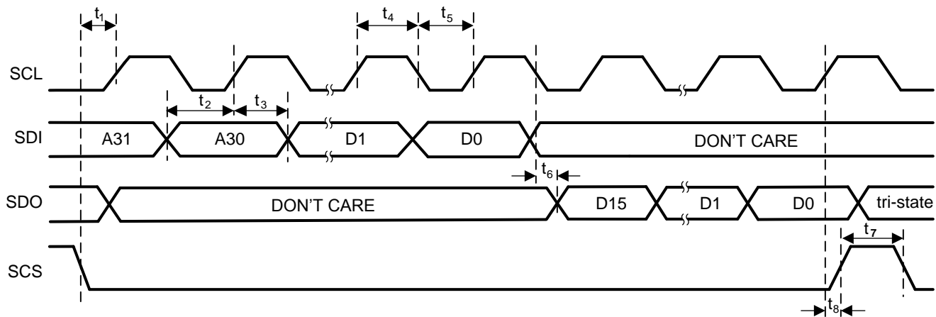
Figure 49. CDCM6208 SPI Port Timing
