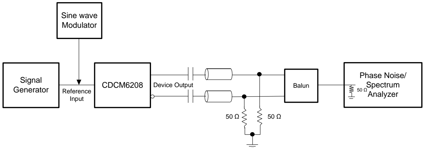
Figure 22. Jitter transfer Test Setup
