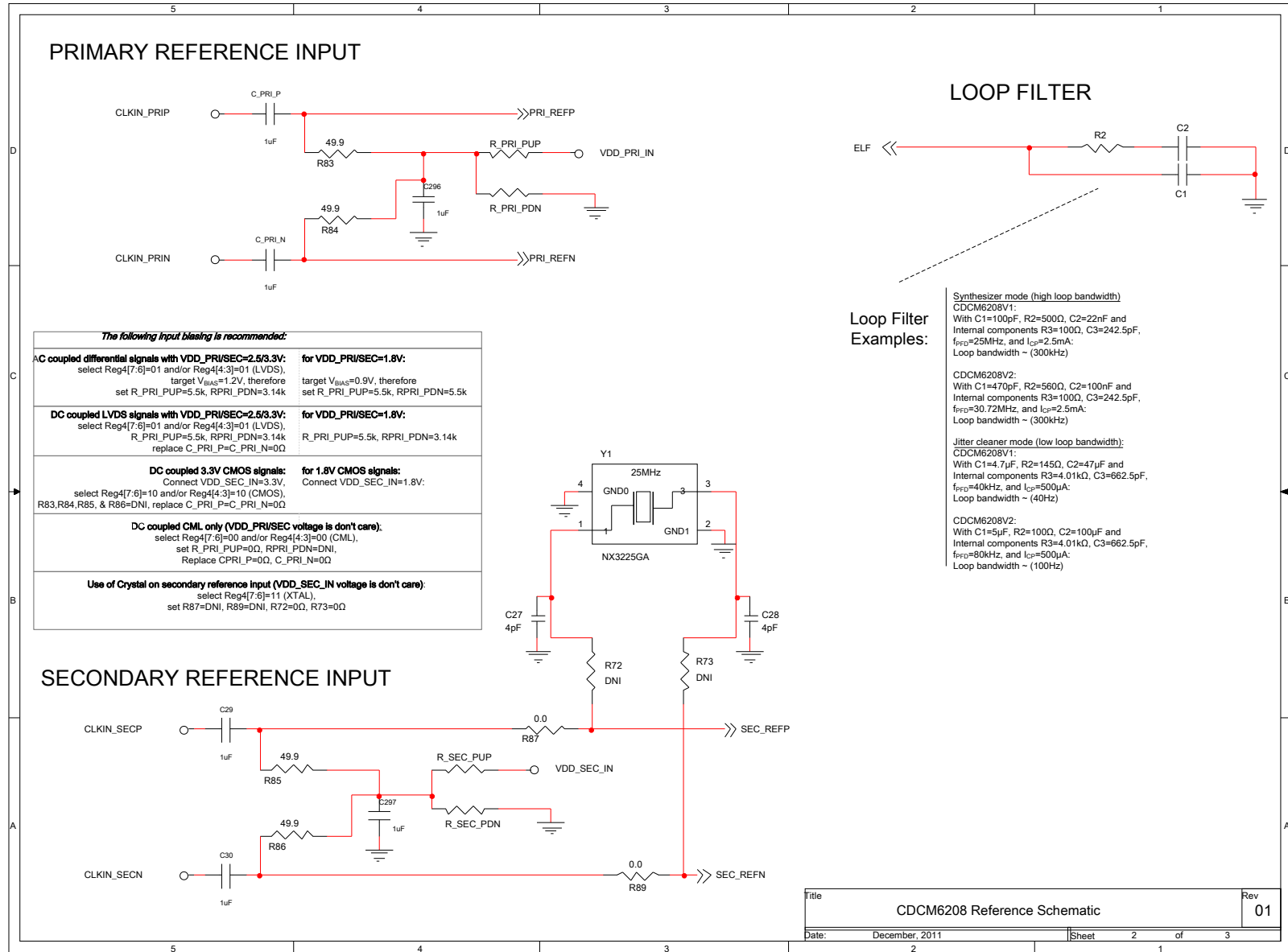
Figure 55. Schematic Page 2
