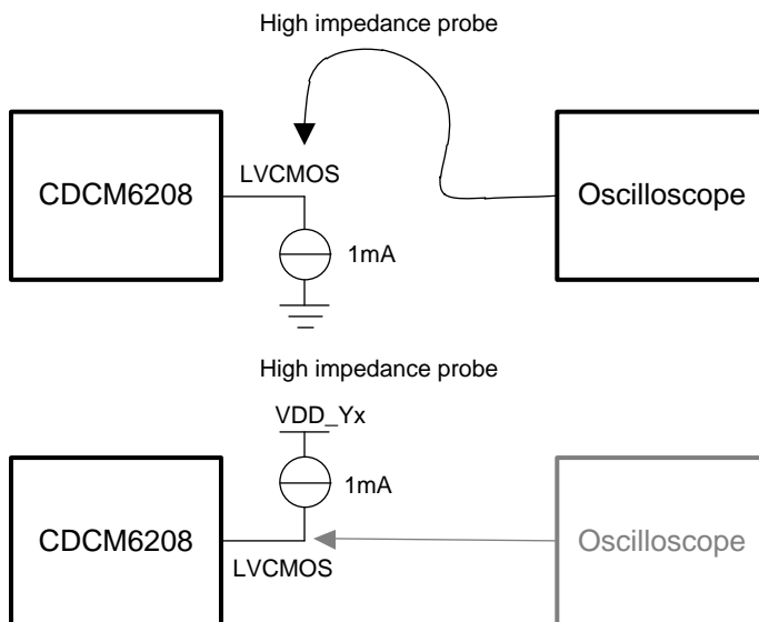
Figure 11. LVC MOS Output DC Configuration During Device Test
