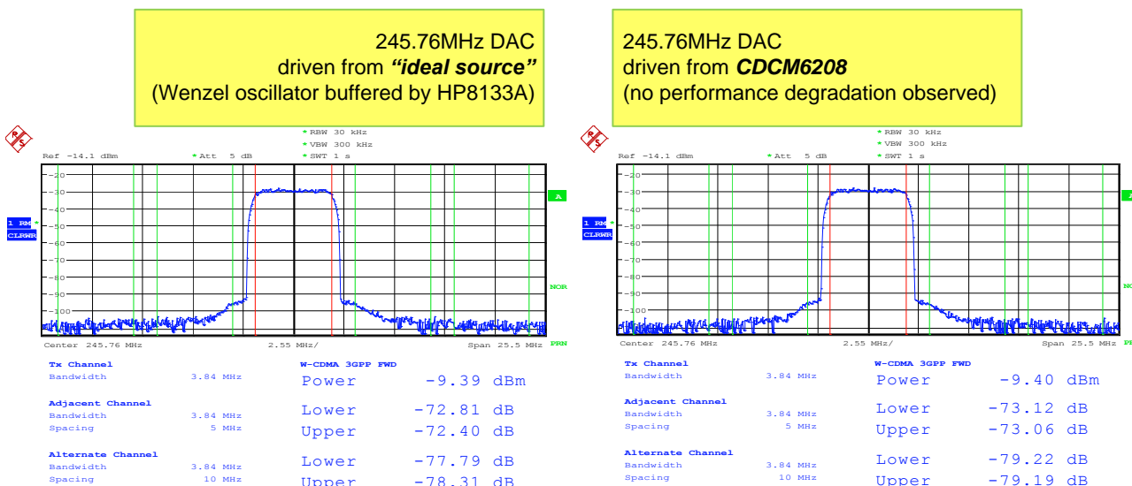
Figure 43. DAC Driven by Lab Source and CDCM6208 in Comparison (Performance Identical)
