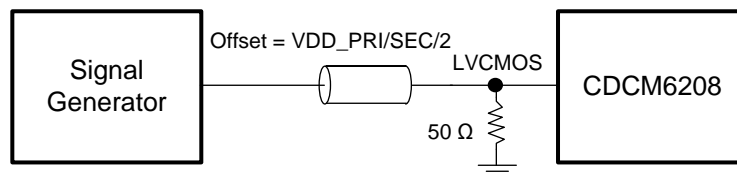
Figure 16. LVCMOS Input DC Configuration During Device Test
