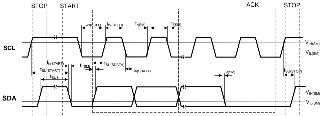
Figure 53. I 2 C Timing Diagram
