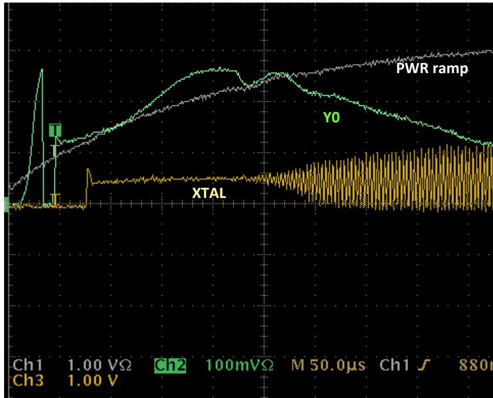
Figure 31. XTAL Startup Using NX3225GA 25 MHz (Step 2)
