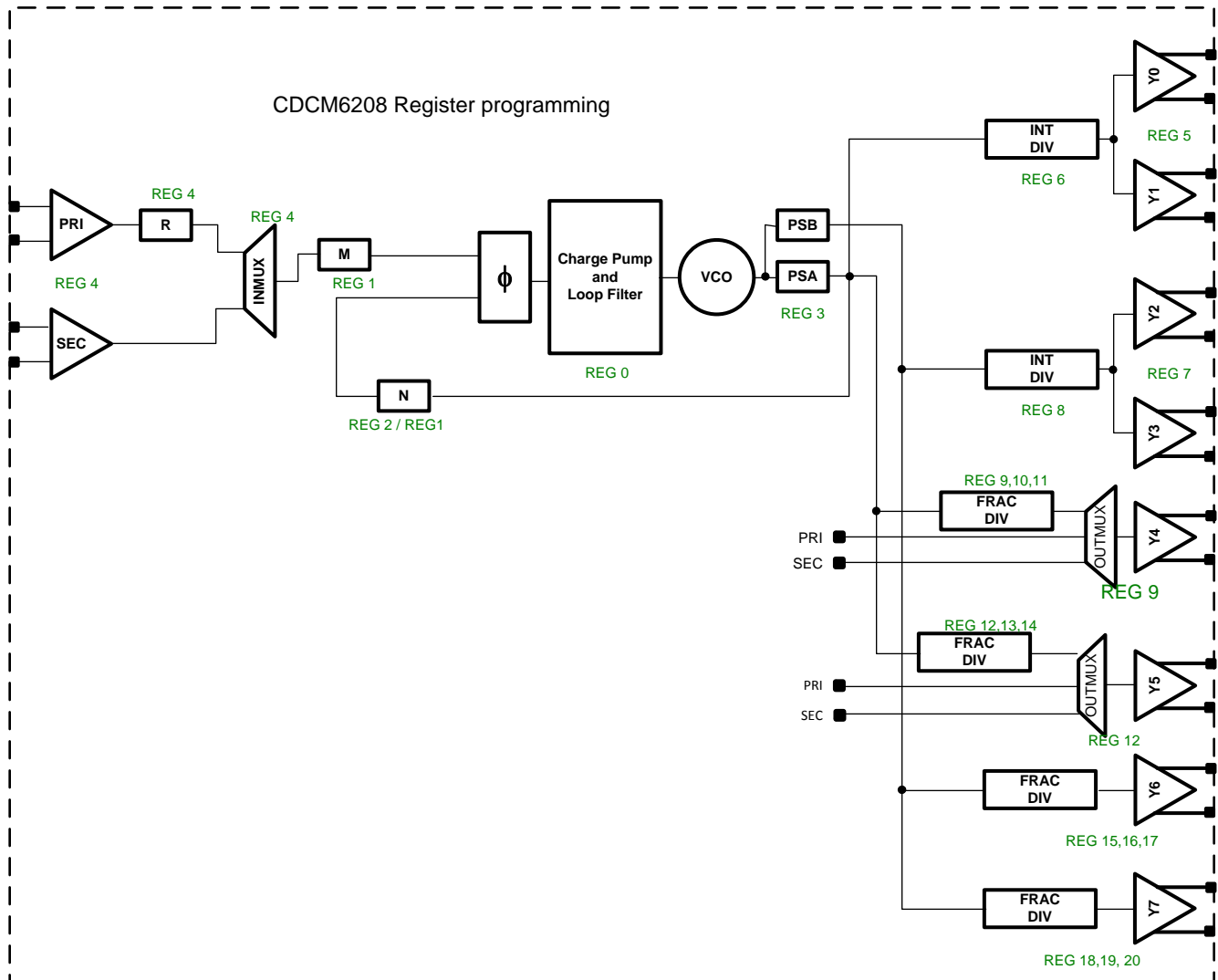
Figure 4. Device Register Map
