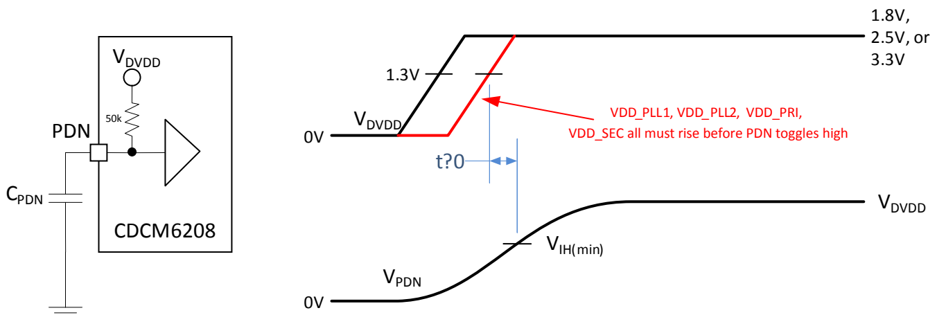
Figure 33. PDN Delay When Using Slow Ramping Power Supplies (Supply Ramp > 50 ms)
