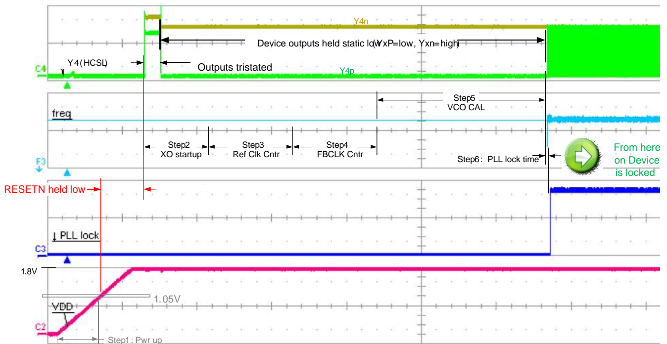
Figure 30. Power up Time
