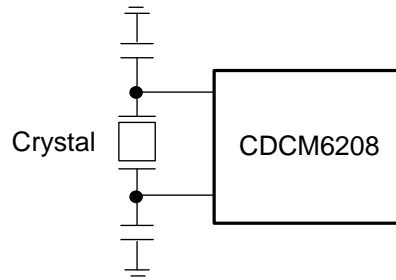
Figure 21. Crystal Reference Input Configuration During Device Test
