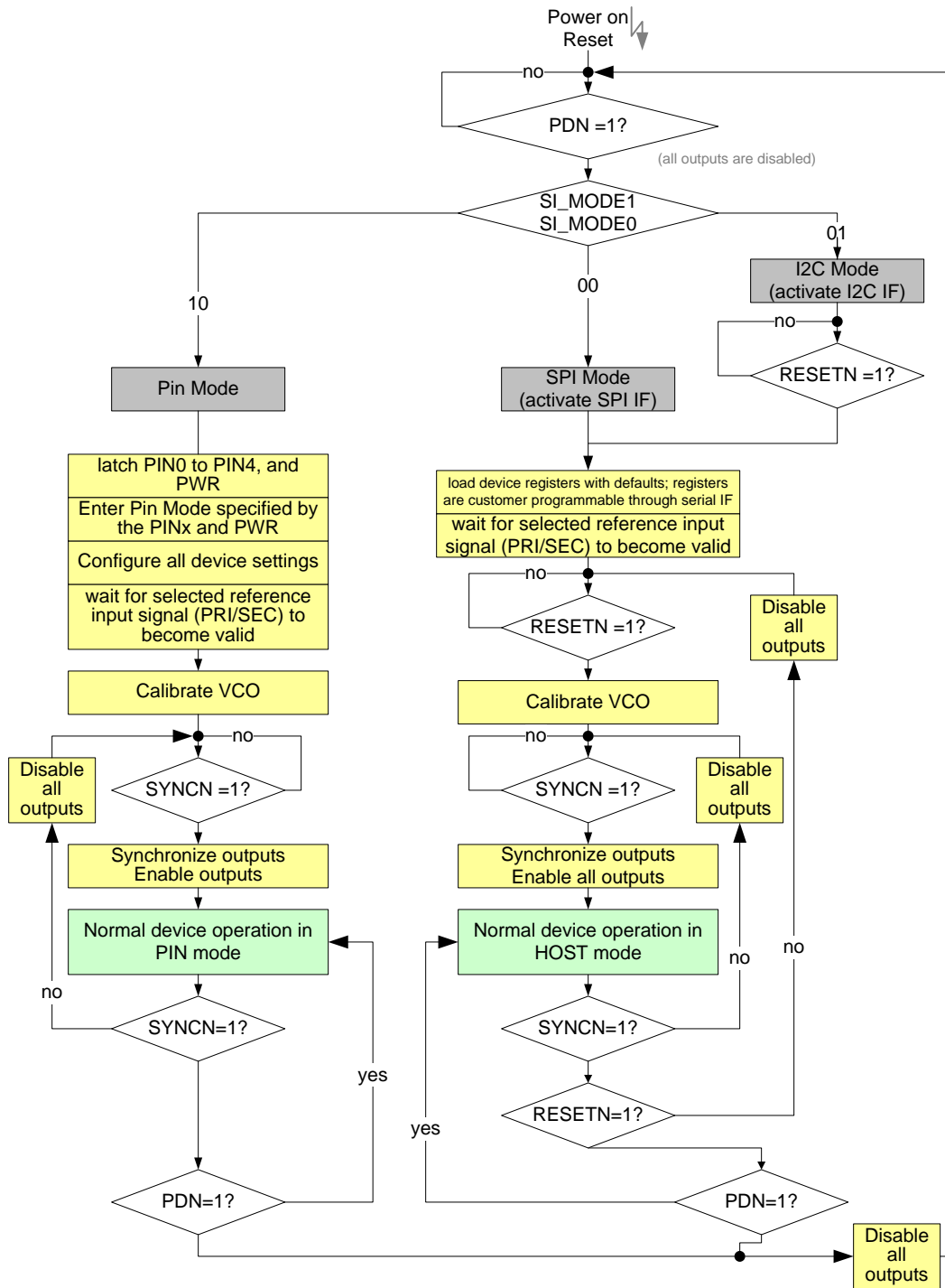
Figure 28. Device Power up and Configuration
