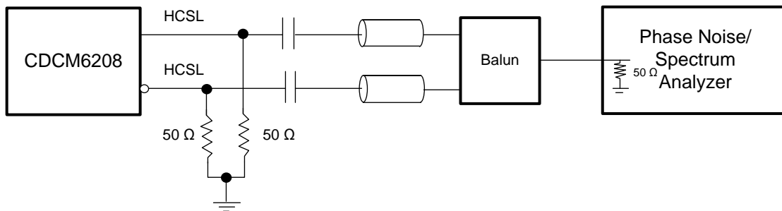
Figure 15. HCSL Output AC Configuration During Device Test
