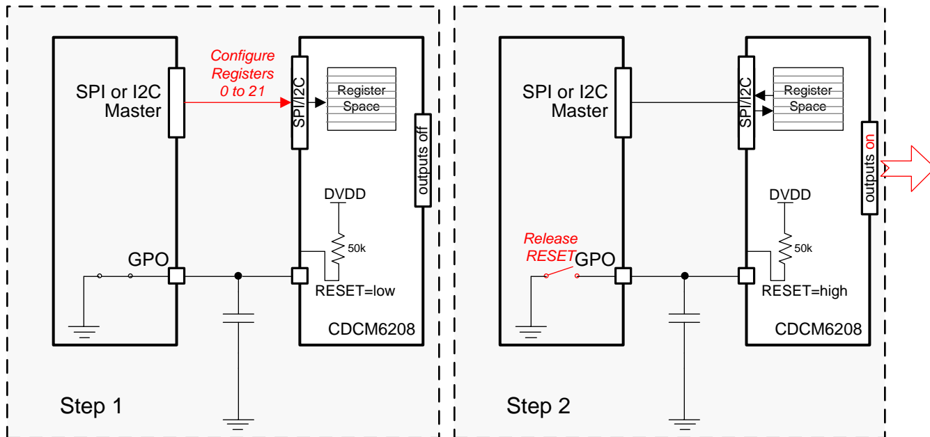
Figure 29. Reset Pin Control During Register Loading
