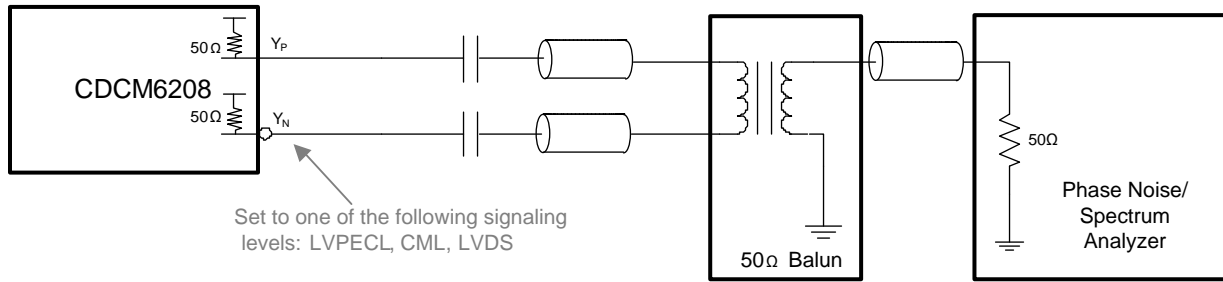
Figure 13. LVDS, CML, and LVPECL Output AC Configuration During Device Test
