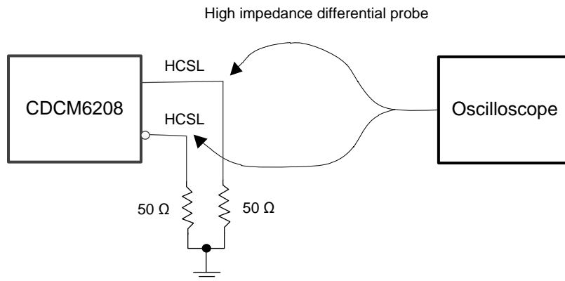
Figure 14. HCSL Output DC Configuration During Device Test
