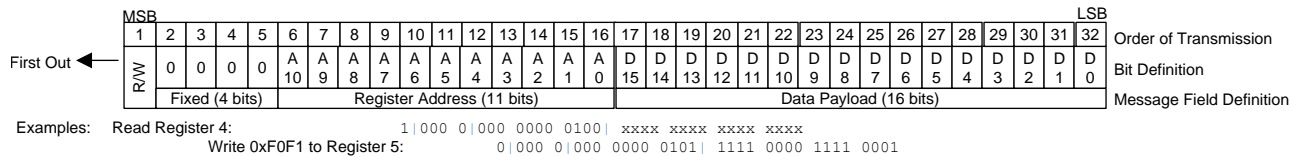
Figure 46. CDCM6208 SPI Message Format
