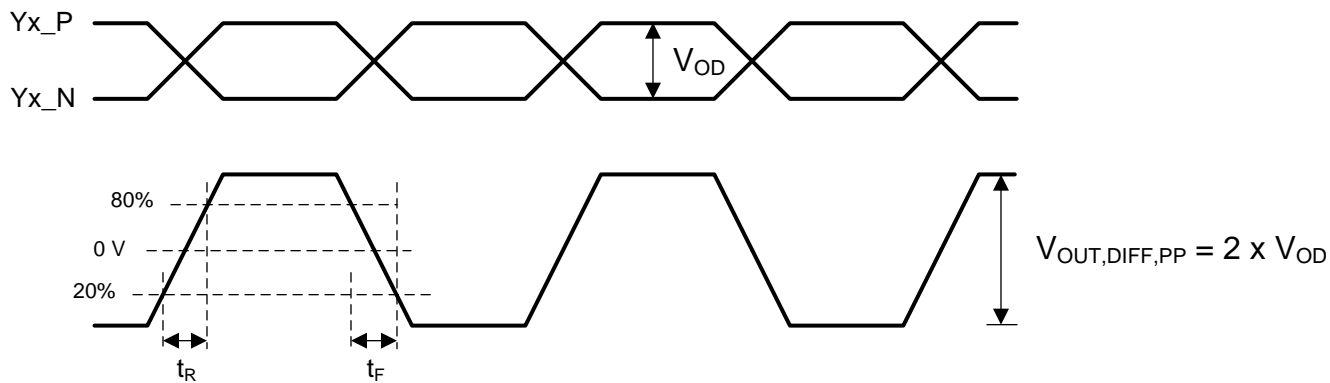
Figure 24. Differential Output Voltage and Rise and Fall Time
